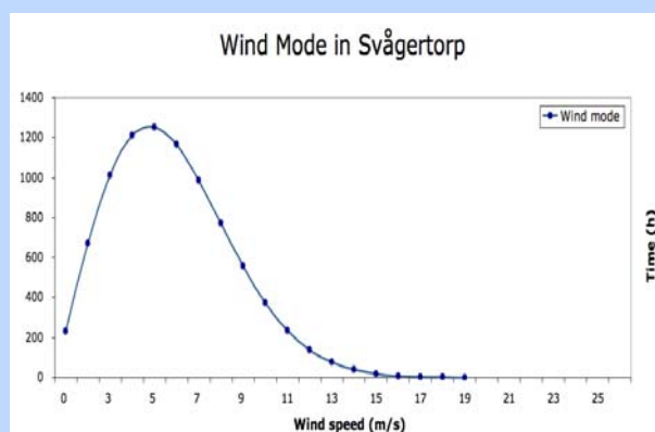
Figure 3 Wind conditions in Svågertorp. Adapted from [9].
