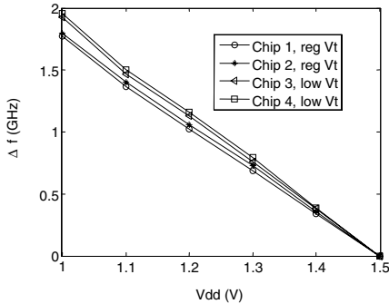
Fig. 10. Oscillator frequency pushing, V_c=0.75\text{V} .
