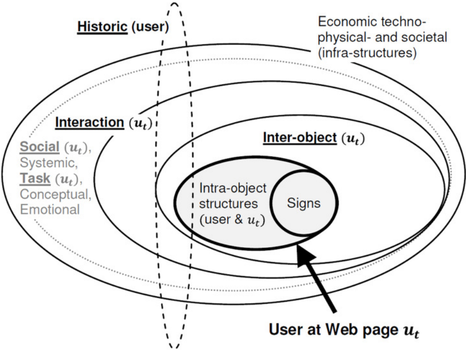
Figure 2. The nested model of context stratification for information seeking and retrieval (based on Ingwersen and Järvelin, 2005).
