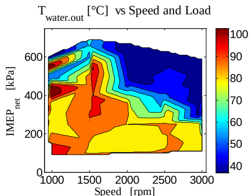
Figure 146: Coolant temperature
