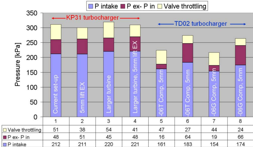
Figure 112: GT-Power turbocharger and valve timing simulation
