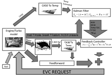
Figure 9. Overview describing the flow of signals as it looks when running the model against the controller. The turbo and the engine models are here combined as Engine/Turbo model.
