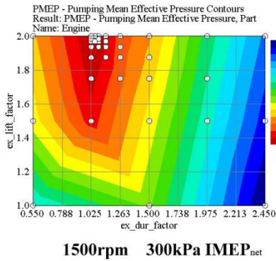
Figure 64: GT-Power simulation
