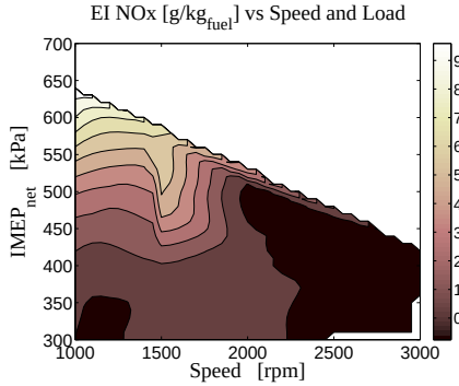
Figure 28: Speed and load testing– NOx emissions
