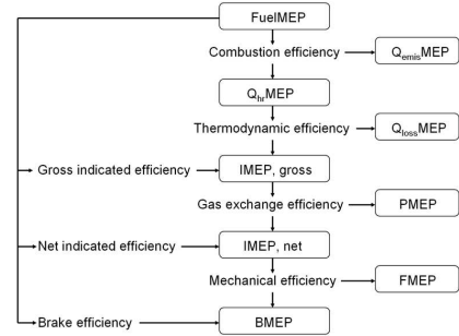
Figure 31: Engine efficiency break-down
