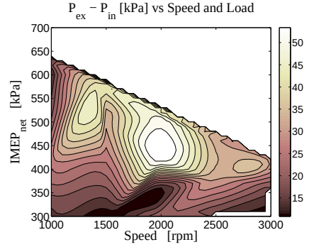
Figure 35: Pressure loss over turbine/compressor: P_{ex} - P_{in}
