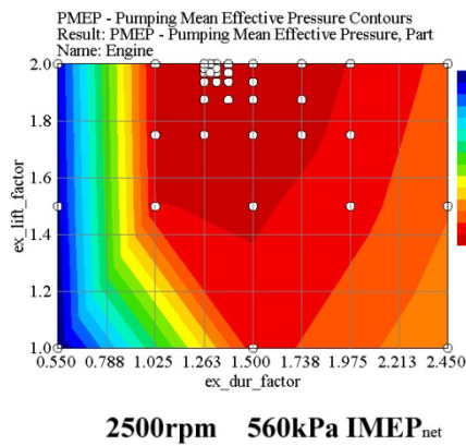
Figure 66: GT-Power simulation
