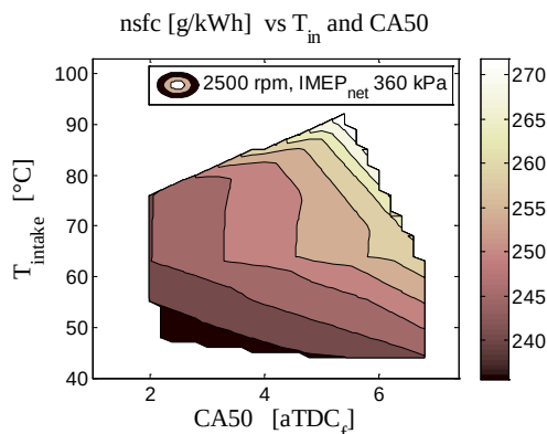
Figure 94: Fuel consumption, nsfc
