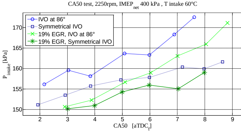
Figure 99: Intake pressure, P_{\text{intake}}
