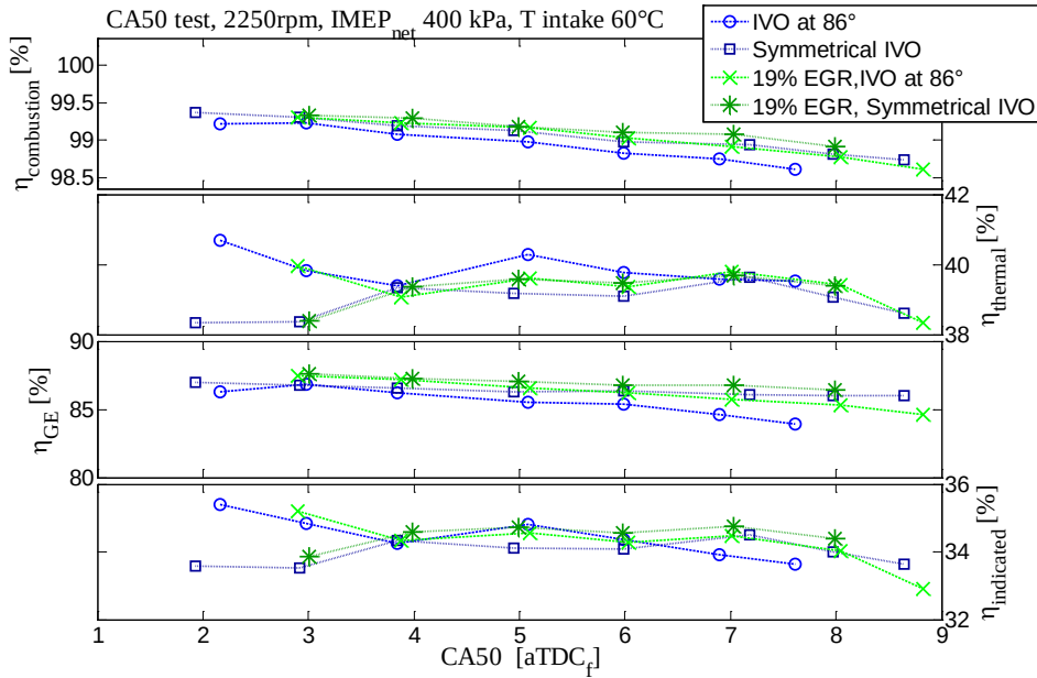
Figure 108: Efficiency breakdown
