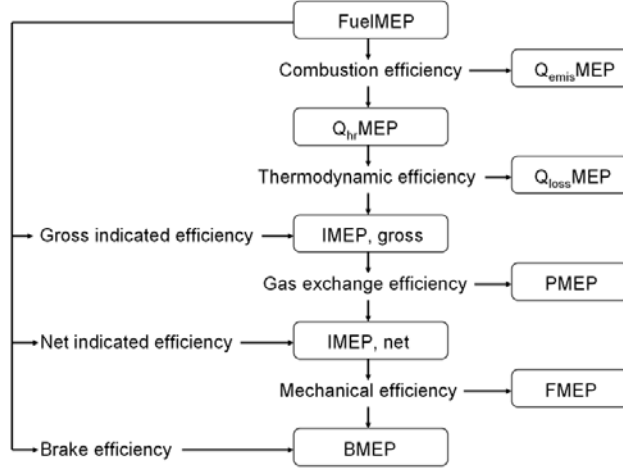
Figure 3: Efficiency breakdown
