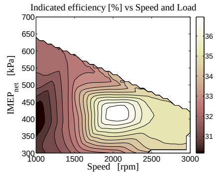
Figure 37: Indicated efficiency
