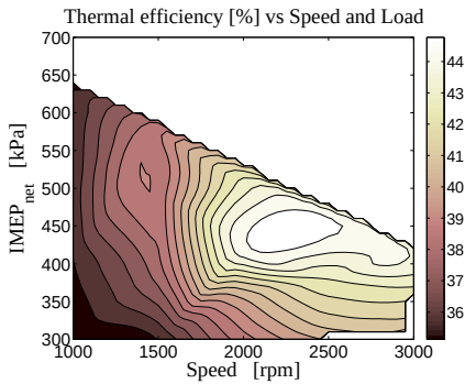
Figure 33: Thermal efficiency
