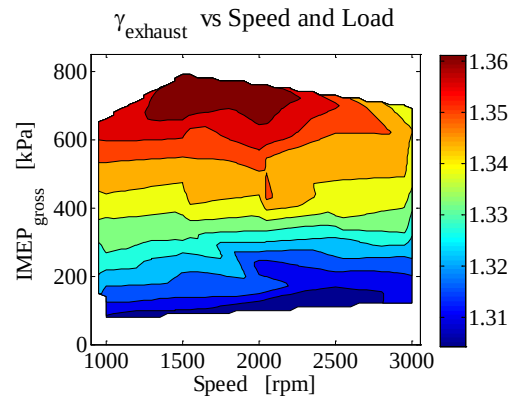
Figure 125: Specific heat ratio, \gamma
