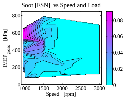
Figure A-3: Soot level, FSN
