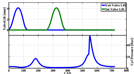
Fig. 1. Valve lift and pressure trace for a NVO HCCI engine
