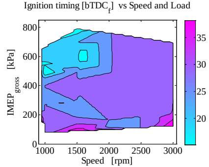
Figure 6: Ignition timing
