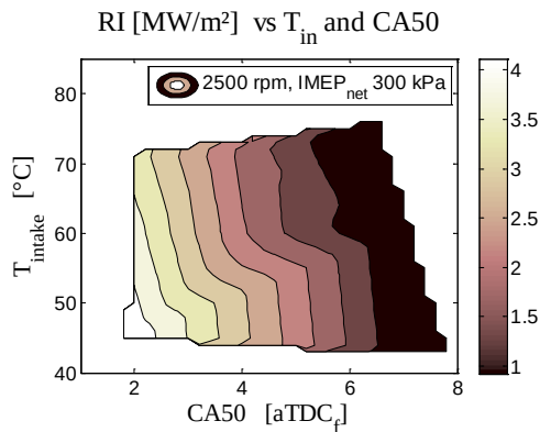
Figure 88: Combustion noise, RI
