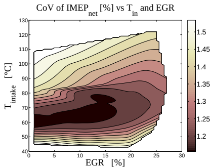
Figure 29: EGR sweep, CoV of IMEP net
