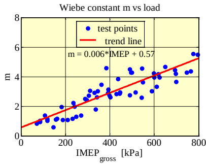
Figure 12: Wiebe constant m vs load
