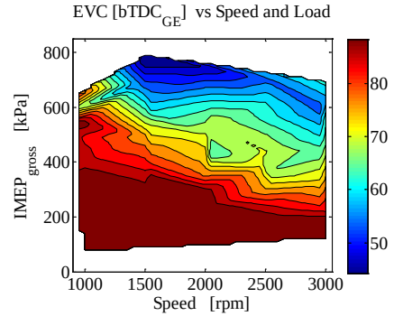
Figure 18: Exhaust valve closing timing, EVC
