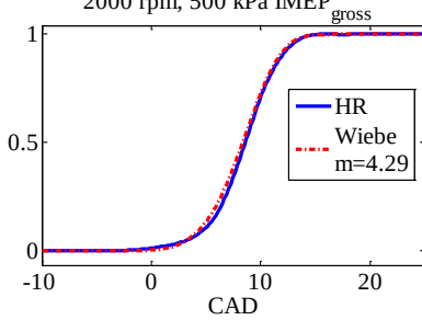
Figure 10: Heat release comparison
