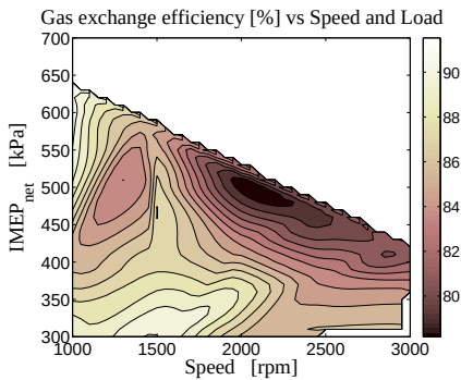
Figure 34: Gas exchange efficiency
