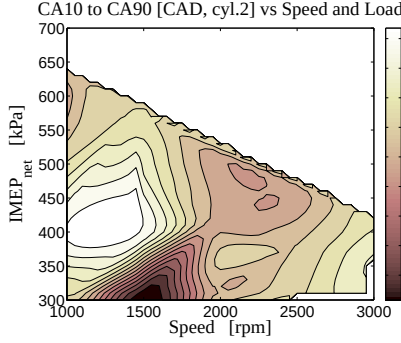
Figure 27: Speed and load testing– CA10 to CA90 duration
