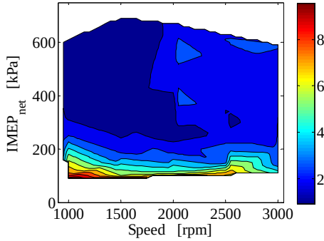
Figure 17: Combustion stability, CoV of IMEP net
