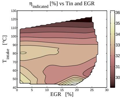
Figure 33: EGR sweep, Indicated efficiency
