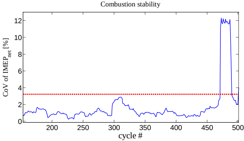
Figure 38: Combustion stability, CoV of IMEP net
