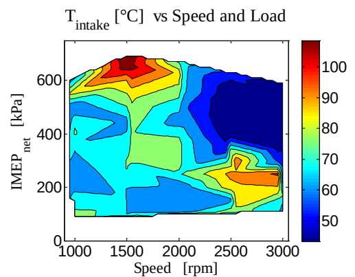
Figure 144: Intake temperature
