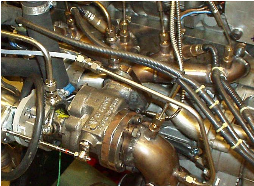
Figure 6: Exhaust manifold
