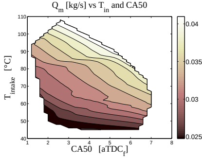
Figure 38: Mass flow
