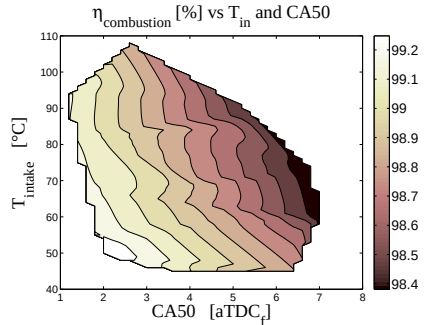
Figure 20: Combustion efficiency
