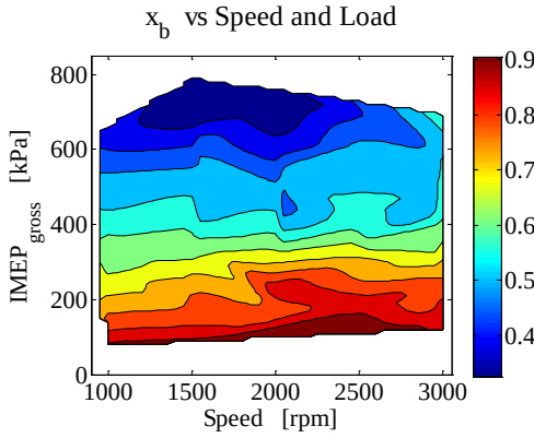
Figure 124: Burned gas fraction, x_b
