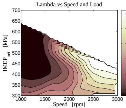
Figure 29: Speed and load testing– Lambda
