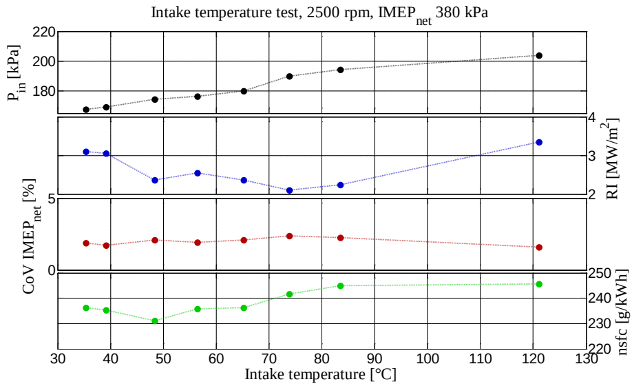
Figure 48: Intake temperature test
