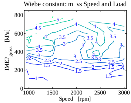
Figure 11: Wiebe constant m vs speed and load
