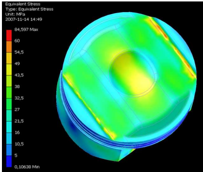
Figure 8: Piston failure FEA
