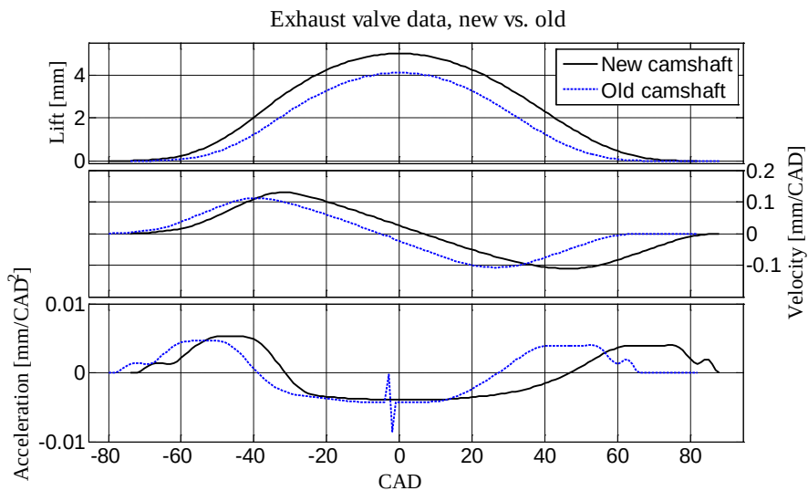
Figure 68: Exhaust valve data comparison
