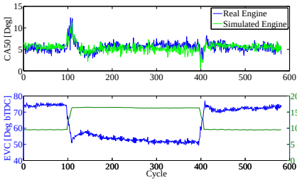
Fig. 7. Validation of model for load steps from low to high to low load at 2000RPM
