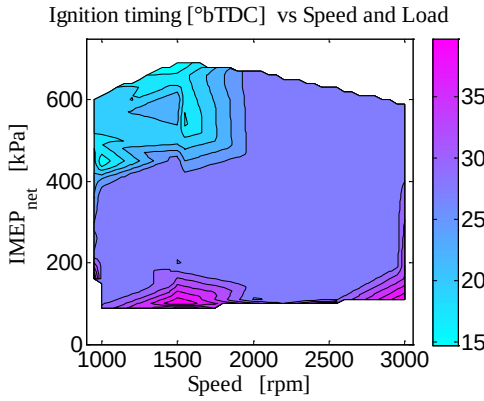
Figure 141: Ignition timing
