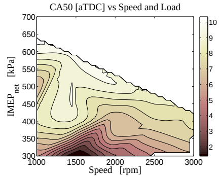
Figure 19: Speed and load testing– CA50 position
