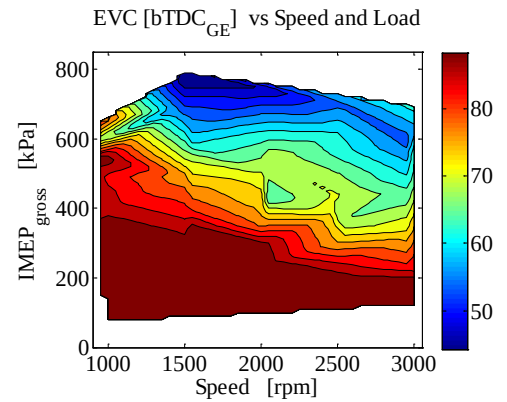
Figure 129: Experimental EVC
