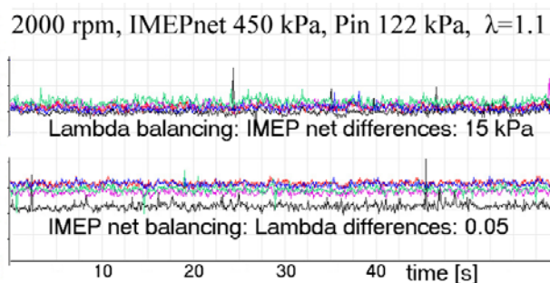
Figure 10: Cylinder individual lambda traces, lambda balancing vs. IMEP balancing
