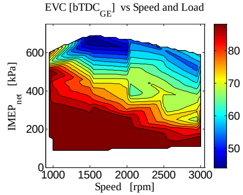
Figure 142: Exhaust valve closing timing
