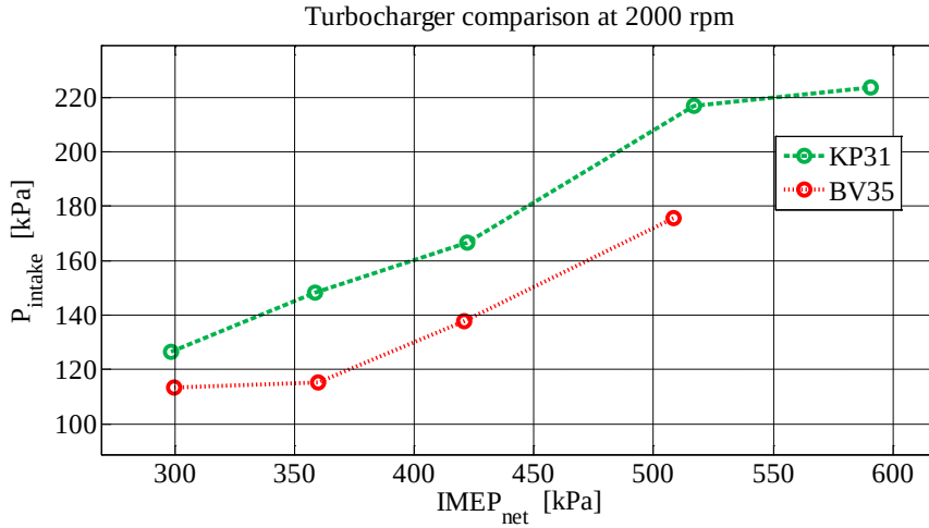
Figure 55: Turbocharger comparison
