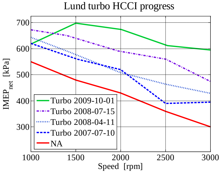
Figure 132: Maximum load range progress
