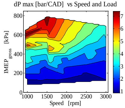
Figure A-6: Maximum pressure rise rate
