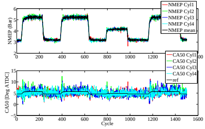
Fig. 11. CA50 during load steps
