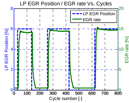
Figure 67 The dynamics of the long route (i.e. LP) EGR system.
