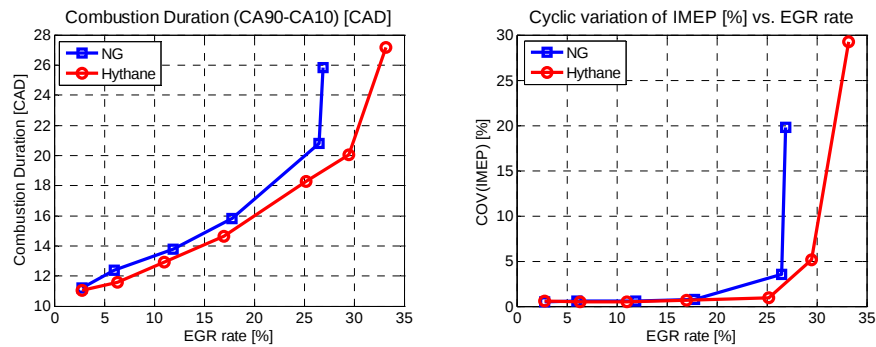
Figure 76 Combustion duration versus EGR rate
