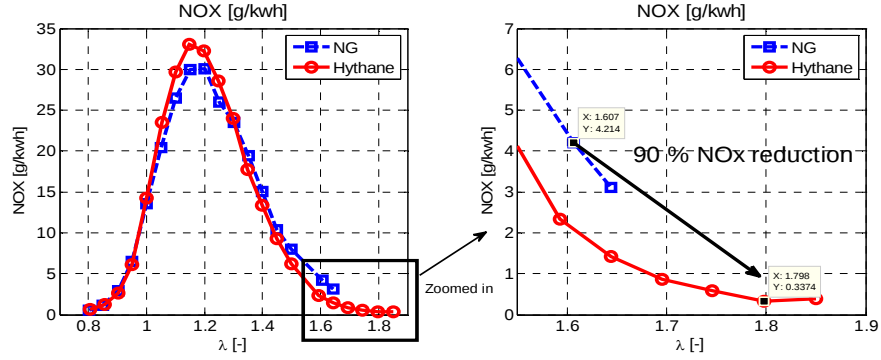
Figure 73 Specific NO x emissions over lambda range for Hythane and natural gas are compared. NO x emissions for operating points close to the lean limit is zoomed in, to clarify the benefits in NO x reduction
