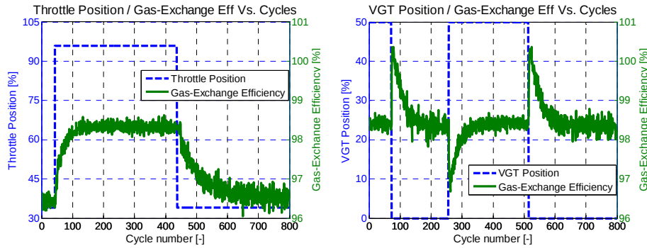
Figure 58 Gas-Exchange efficiency as throttle used to control the desired load at 1400 RPM Figure 59 Gas-Exchange efficiency as VGT used to control the desired load at 1400 RPM
