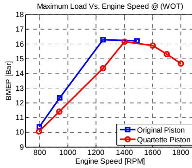
Figure 46 Maximum Load at different engine speed (WOT)
