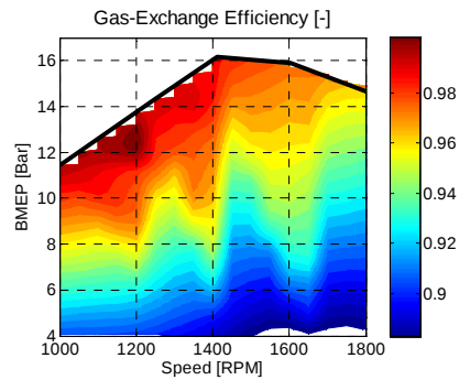
Figure 81 Gas-Exchange efficiency map with natural gas operation
