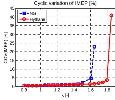
Figure 69 COV(IMEP) versus lambda
