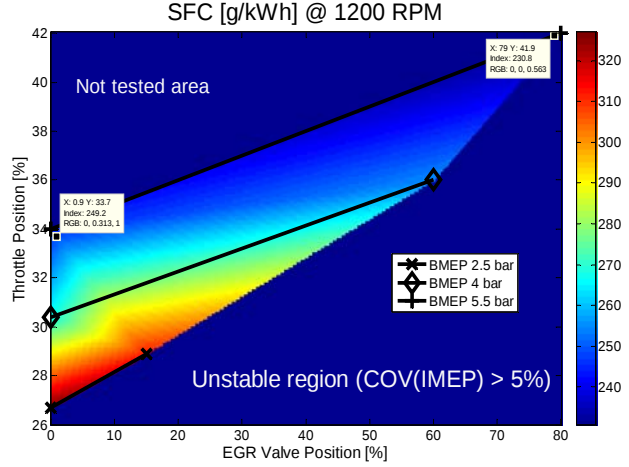
Figure 30 SFC reduces as a result of more throttle opening
