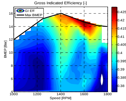
Figure 84 Gross-Indicated efficiency map with Hythane
