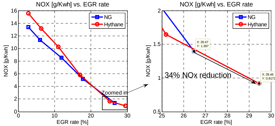
Figure 78 Specific \text{NO}_x emissions over EGR range for Hythane and natural gas are compared. The operating region close to dilution limit is zoomed in to the right, to clarify the benefits in \text{NO}_x reduction.
