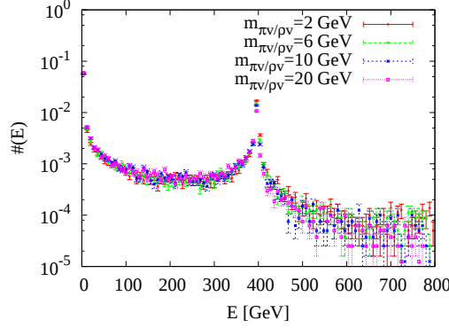
Figure IV.11: KMNA_{\gamma\nu} : The total energy radiated in ISR photons. Note the spike around 400 GeV: a large fraction of the events will have a reduced \hat{s} due IS photon emission. The q_\nu mass is fixed by m_{q_\nu} = m_{\pi/\rho_\nu}/2 .
