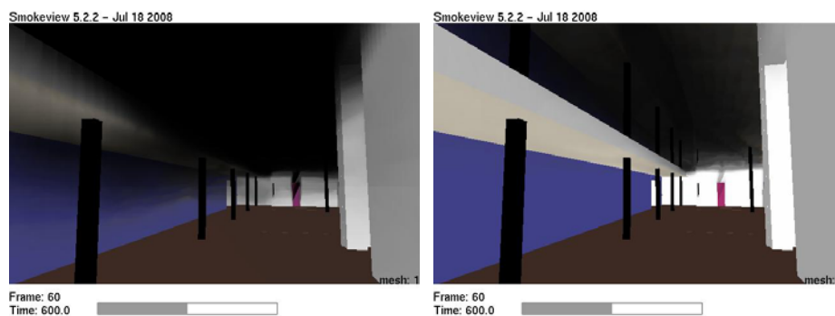
Figure 16. Comparison of soot concentration at 600s between cable M (left) and cable I (right)
