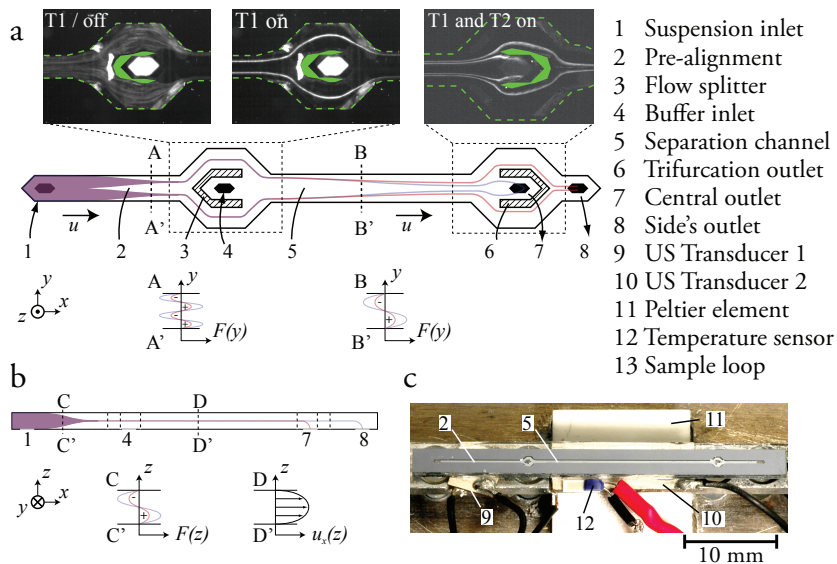
of cells or microbeads. (a) Top view schematic of the channel, and (b) side view schematic. (c) Photo of the device.
