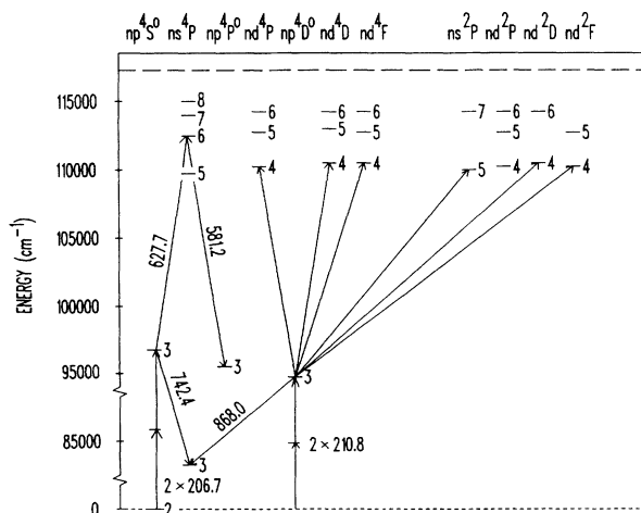
FIG. 1. Energy-level diagram for the nitrogen atom, with excitation pathways indicated (wavelengths in nm).
