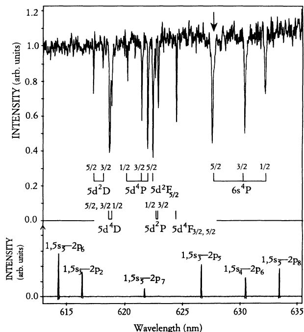
FIG. 4. Depletion spectra for nitrogen obtained by scanning a second-step dye laser inducing single-photon transitions from the 2p^2 3p^4 S platform state, the population depletion of which is monitored on the 742-nm line. The lower part shows a neon spectrum with original Paschen notation.
