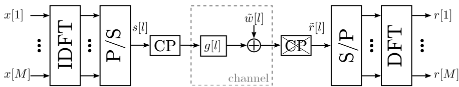
Figure 2.1: A baseband OFDM system model.
