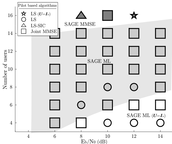
Figure 8: The algorithm combinations with the lowest total complexity, reaching a BER=10 -3 , at different user numbers and E_b/N_0 . Shape indicates which pilot based algorithms were used, and color indicates which decision-directed algorithms that were used. The system settings are S_p = 1 and S = 20 OFDM symbols, M = 256 subcarriers and I = 27 DPS sequences.
