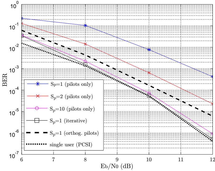
Figure 3.3: The BER at different SNR for a MU-MIMO system with N = 4 receive antennas and K = 4 users. Different number of pilot OFDM symbols are used, S_p = 1, 2 and 10 , where the total number of symbols is S = 20 . Also shown is the performance obtained when using the channel estimator in the loop of the iterative receiver, as well as single user performance when the channel is perfectly known, and the case of orthogonal boosted pilots. (From Paper I.)
