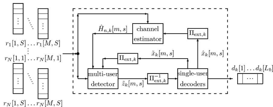
Figure 3: The structure of the iterative receiver.
