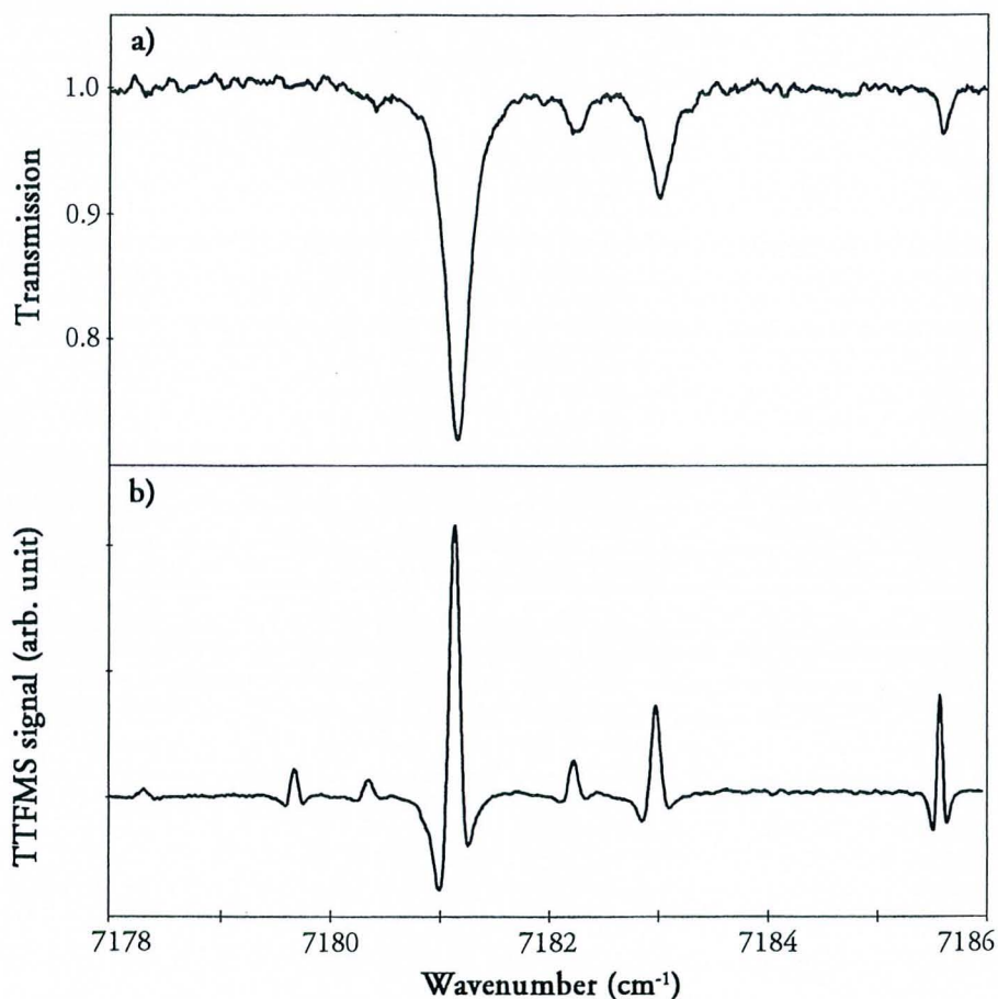
Fig. 4.4 a) Direct absorption and b) TTFMS spectra of water vapour around 1.39 \mu\text{m} measured over a pathlength of 0.5 m in indoor air (relative humidity \approx 40\% ). The integration time for the two spectra is the same.
