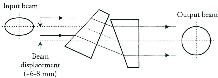
Fig. 2.2 Schematic illustration showing the working principle of an anamorphic prism pair. The prism pair transforms an elliptical beam into a circular beam, either by expanding, or decreasing the beam in one direction only. The prism pair shown here expands the minor axis to make a circular beam. The transformation is always accompanied by a small displacement of the beam. The amount of magnification (or demagnification) can be varied by changing the incident angle. The two identical prisms are mounted with an incident angle close to Brewster's angle to minimise reflection losses and maintain the state of polarisation.
