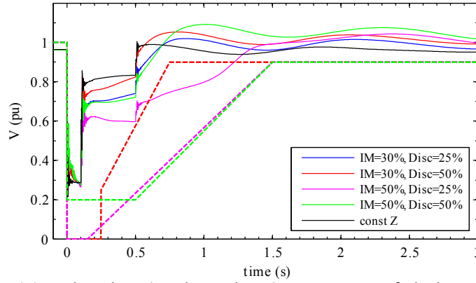
Figure 6.6 Fault on line 6-7a close to bus 6, Case 2. Correct fault clearing. Swedish (red dashed), E.ON (magenta dashed) and Danish (green dashed) GFRT curve.
