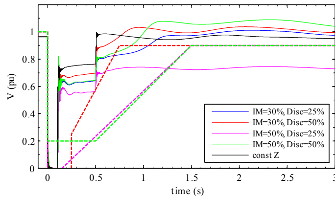
Figure 6.8 Fault on line 1-6a close to bus 1041, Case 3. Correct fault clearing. Swedish (red dashed), E.ON (magenta dashed) and Danish (green dashed) GFRT curve.
