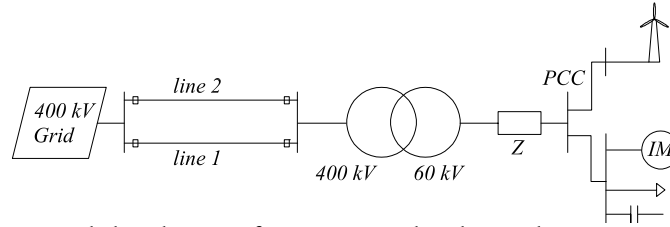
Figure 7.5 Single-line diagram of test system used in the simulations.
