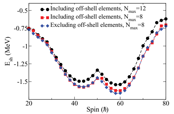
FIG. 6. (Color online) The shell energy for the configuration [8(22), (22)6(11)] with deformation parameters \varepsilon_2 \sim 0.43 , \gamma \sim 20^\circ , and \varepsilon_4 \sim 0.028 in the ^{168}\text{Hf} nucleus. The circles show the calculations including the off-shell elements and \mathcal{N}_{\text{max}} = 12 , the squares include the off-shell elements and \mathcal{N}_{\text{max}} = 8 , and the diamonds exclude the off-shell elements and \mathcal{N}_{\text{max}} = 8 .
