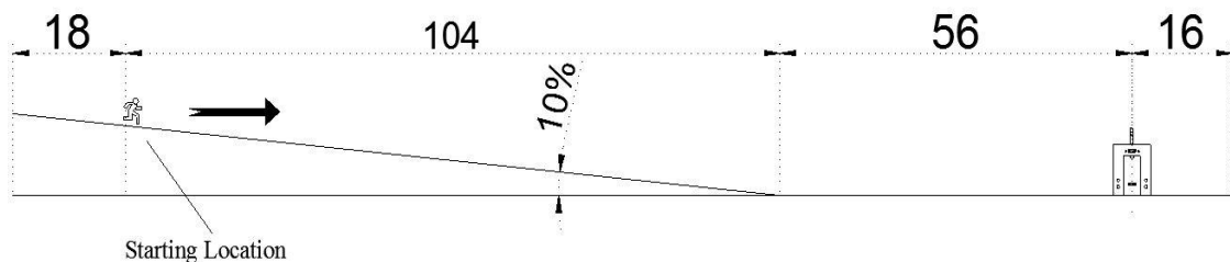
Figure 2 . Side view of the Träskolevägen tunnel.
