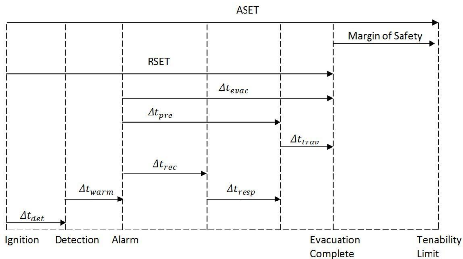
Figure 3. Egress time-line
