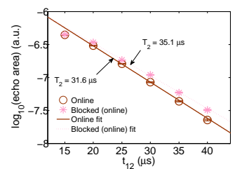
Figure 7.10. Echo decay curve from the Pr:Ce: Y_2SiO_5 crystal.
