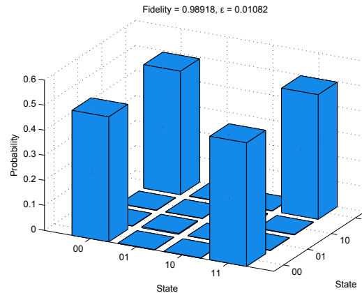
FIG. 4. (color online) Shows the (real) elements of the density matrix of a prepared Bell state, including all error sources described in the text. The total fidelity without readout 99.3% and with readout 98.9%.
