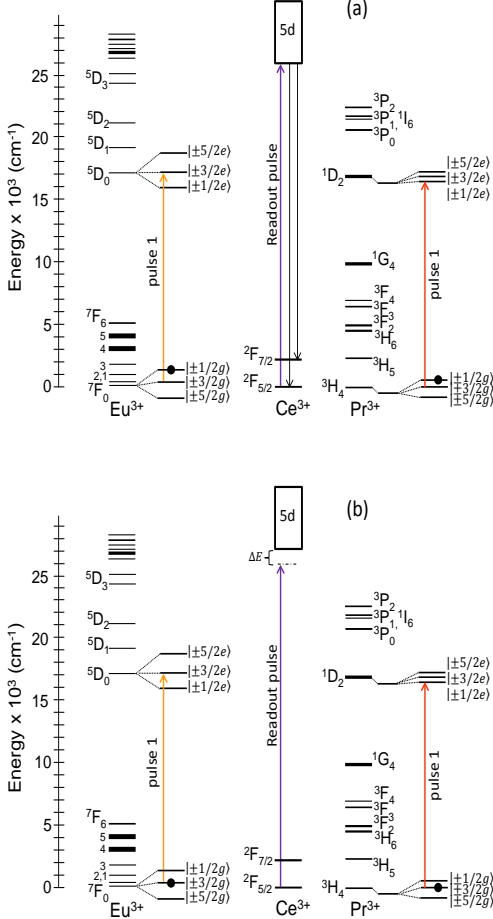
FIG. 1: Ce^{3+}-Pr^{3+}/Eu^{3+} readout scheme. Solid colored arrows represent the excitation pulses at approximately 370 nm, 606 nm and 580 nm for Ce^{3+} , Pr^{3+} and Eu^{3+} respectively. (a) Ce^{3+} emission should be detected when the qubit ion is initially found in the state |1/2g\rangle . (b) No emission is expected from the Ce^{3+} ion when the qubit is in the ground hyperfine state |3/2g\rangle . The hyperfine splitting of the {}^7F_0 and {}^5D_0 Eu^{3+} singlets and the lowest stark level of the {}^3H_4 and {}^1D_1 Pr^{3+} multiplets are not scaled in energy to the spin-orbit electronic levels as it is just several MHz ( 10^{-3} cm ^{-1} ) in the case of Pr^{3+} and hundreds of MHz for Eu^{3+} ( 10^{-2} cm ^{-1} ).
