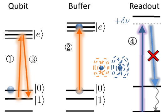
FIG. 2. (color online) Pulse sequence for reading out the state of one qubit via one buffer ion and the readout ion. In the instance shown the qubit is in |0\rangle state, which means the buffer ion gets excited, shifts the readout, which in turn stops fluorescing. If the ion instead was in the |1\rangle state, the buffer would be shifted, and would thus not become excited, and the readout would fluoresce normally.
