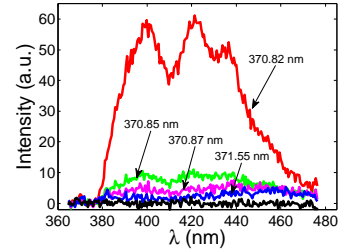
Figure 8.14. The fluorescence spectra recorded at different excitation wavelengths as indicated in the figure. The black curve is the background signal when the excitation laser is blocked.
