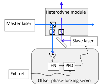
Figure 5.13. Schematic diagram of the offset phase-locking scheme.
