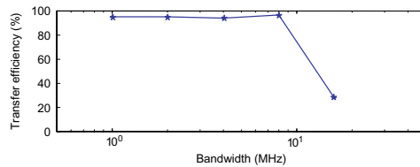
Figure 7. Transfer efficiency of |0\rangle \rightarrow |e\rangle by means of optimal control pulses as a function of bandwidth.
