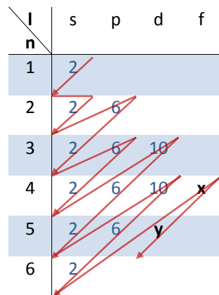
Figure 3.1. Electron distribution of RE elements in different subshells. Arrows indicate the filling order of the electrons. More information is given in the text.
