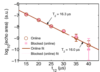
Figure 7.9. Echo decay curve on the Pr ions in an Y_2SiO_5 crystal.
