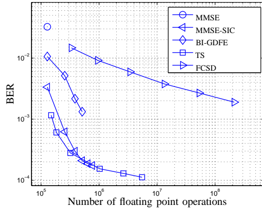
Fig. 13. Comparisons of BER of the studied detectors as functions of their complexities given in Table II. We consider the case without possibility of pre-processing, i.e., the column entries in Table II are summed for each scheme. The number of antennas M = K = 40 , and transmit signaling power \rho = 12 dB.
