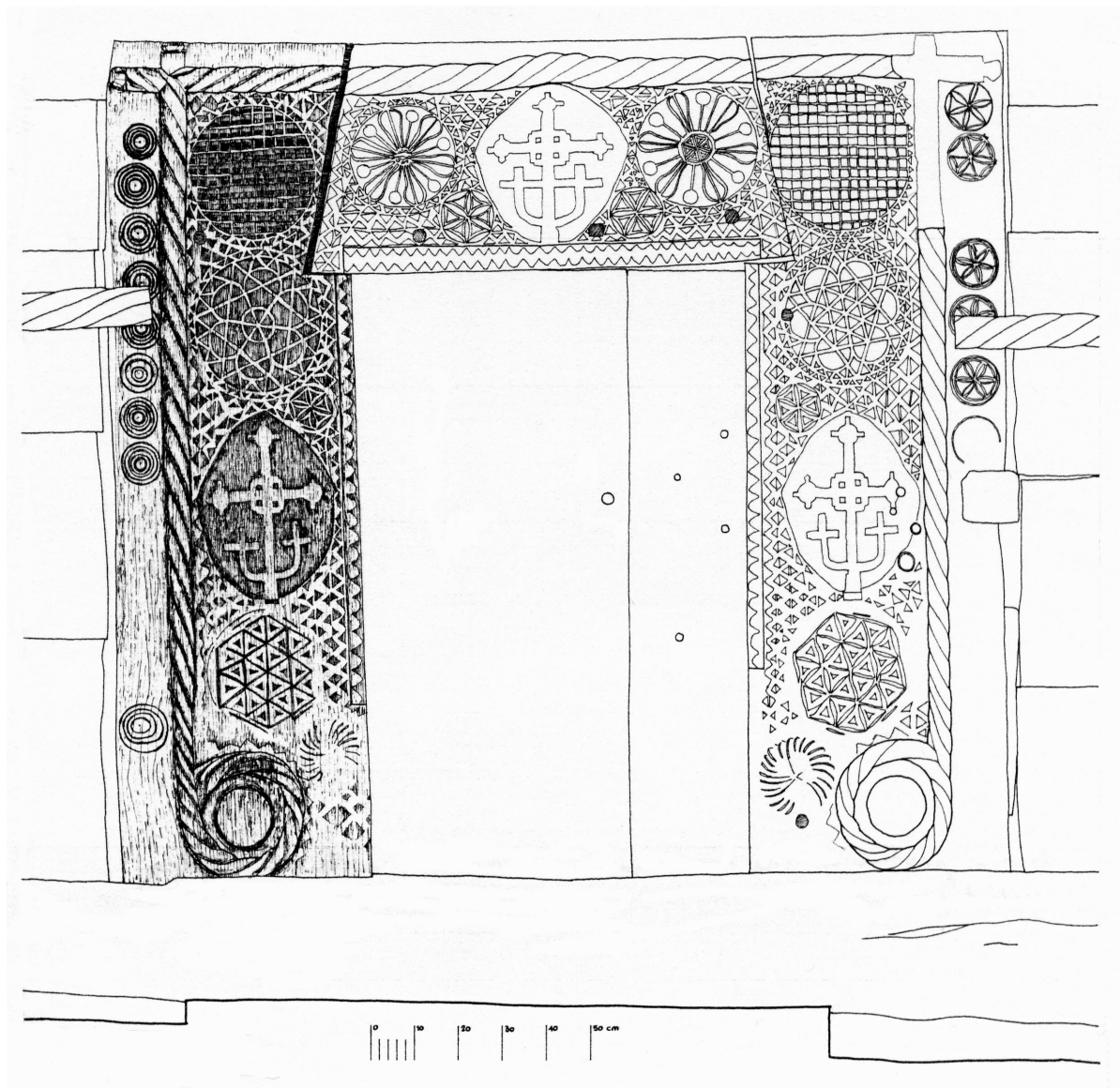
173 Sârbi Susani. The portal of the entrance (1639) is a masterpiece of vernacular Christian art and a distinctive professional mark that provides us with some essential keys to understand the symbolical language of the carpenters. Scale drawing and tracing 1:20, April 1995.
