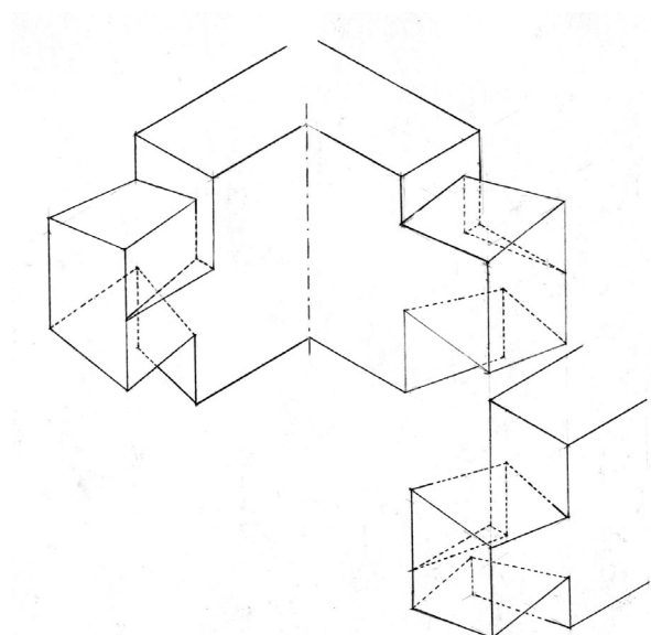
56 Poienile de sub Munte . A particular type of dovetail joint with a recess inside. Scale drawing: June 1998.
