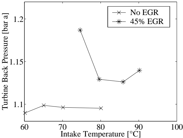
Figure 24. Turbine backpressure with and without EGR at turbo charged condition.
