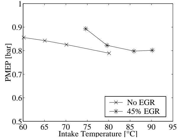
Figure 22. PMEP with and without EGR at turbo charged condition. 11 bar BMEP at 1600 rpm
