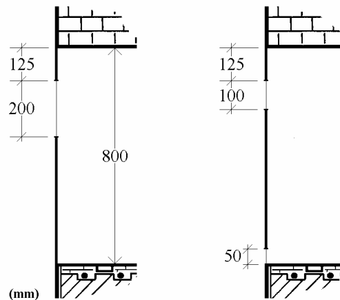
Figure 2. Opening configurations used in the combustion chamber. The left one was used in test 001-021 and the right was used in test 022-038
