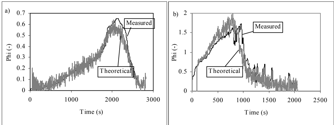
Figure 2. A comparison between measured and calculated \phi -values for an experiment with a) TMTM in the 1/3 scale ISO room and b) for heptane in the 1/3 scale ISO room.
