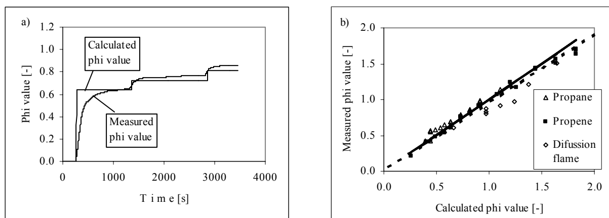
Figure 3. a) Measured and calculated phi values from an experiment on the combustion of propane, as a function of time. b) Experimental versus calculated phi values for measurements with the phi-meter. Results for propane, propene and a propene diffusion flame are shown in the diagram. The solid straight line represents the ideal results when measured and calculated values are equal and the dotted line represents the result of linear regression which gives a constant of determination R^2=0.950 .
