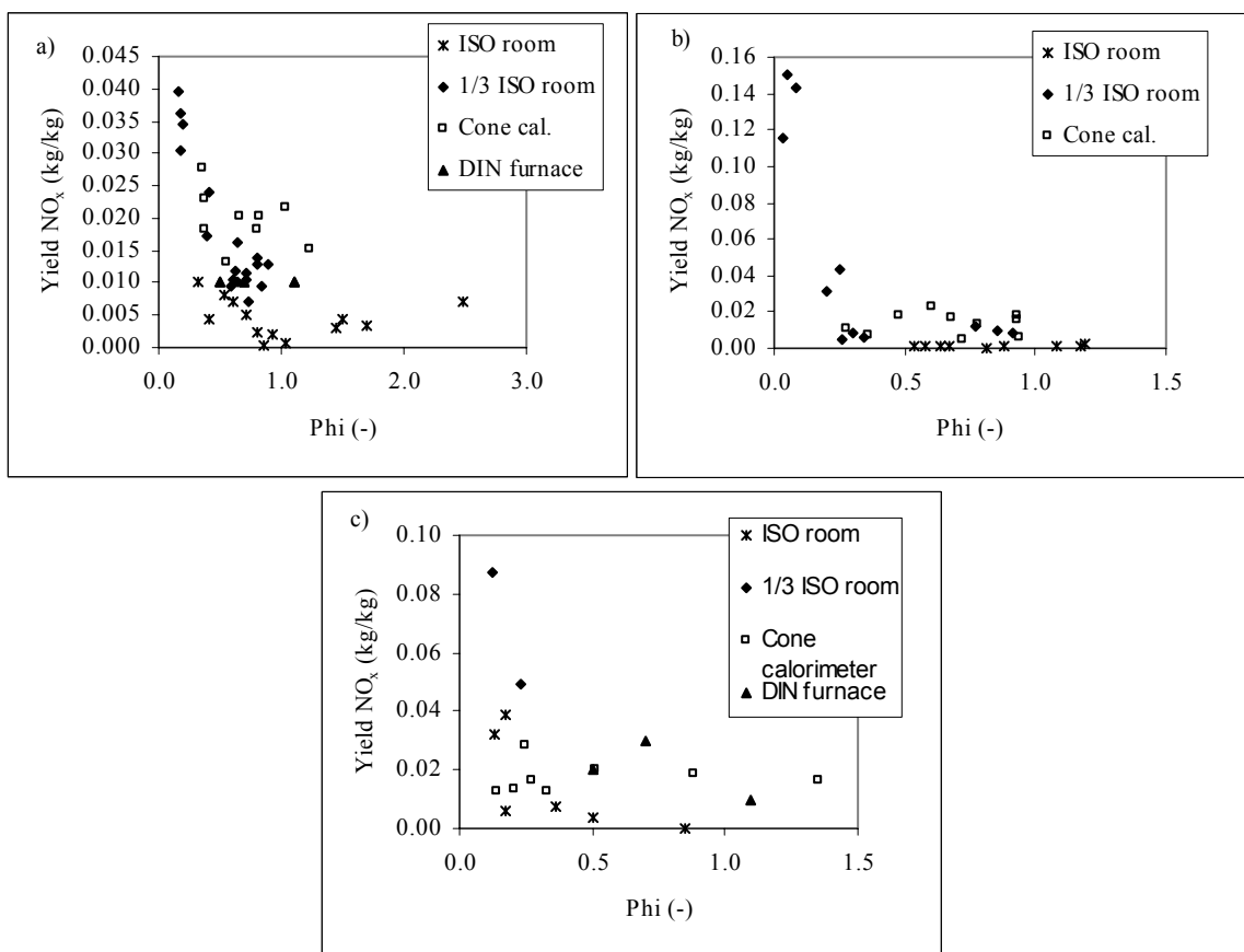
Figure 10 a) The yield of \text{NO}_x from experiments with TMTM as a function of the \phi -value for experiments in the ISO room, the 1/3 ISO room, the cone calorimeter and the DIN furnace. b) The yield of \text{NO}_x from experiments with Nylon as a function of the \phi -value for experiments in the ISO room, the 1/3 ISO room and the cone calorimeter. c) The yield of \text{NO}_x from experiments with CNBA as a function of the \phi -value for experiments in the ISO room, the 1/3 ISO room, the cone calorimeter and the DIN furnace.
