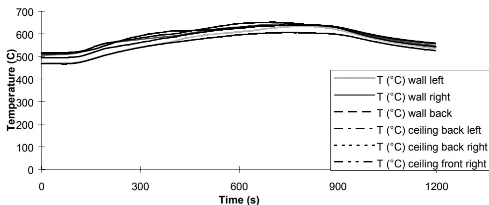
Figure 11. Surface temperature inside the combustion chamber for NYL035 with nylon6,6.
