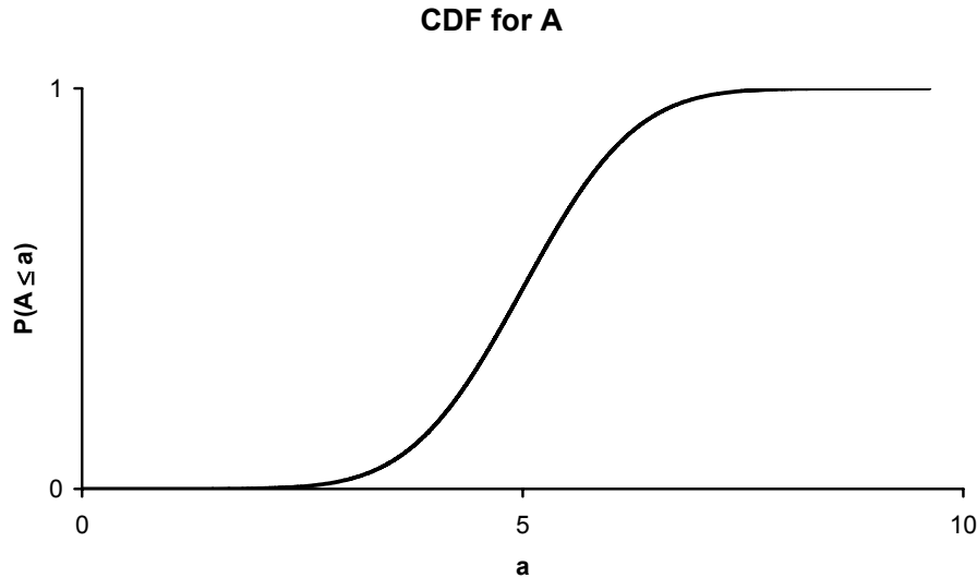
Figure 3.7. Probability distributions are often used to represent uncertainty regarding a quantity. The quantity A is assumed to be normally distributed with mean = 5 and standard deviation = 1. Here, the distribution for A is presented as the Cumulative Distribution Function (cdf).
