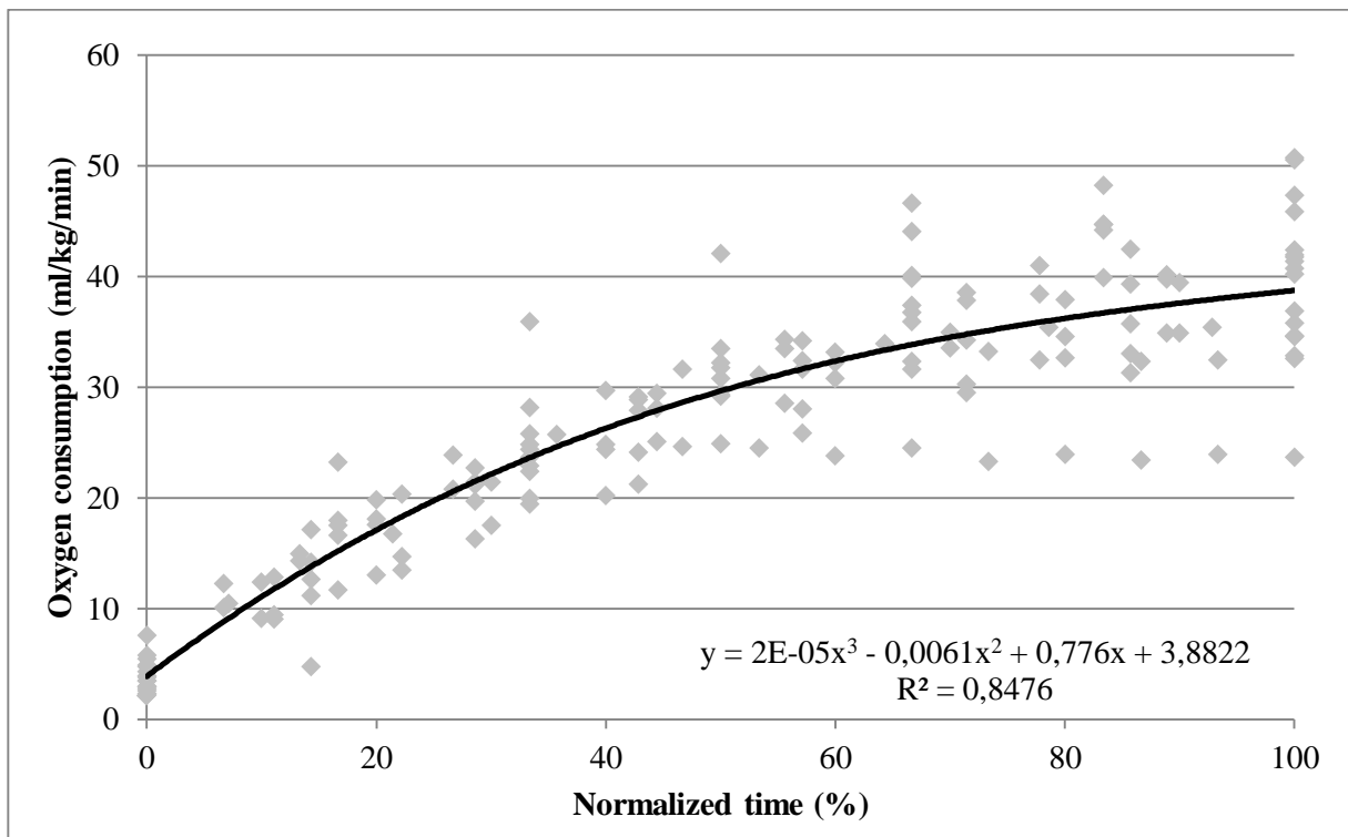
Figure 73. Time normalized development of oxygen consumption in the Västra Skögen experiment. The black line represents a polynomial trend line.
