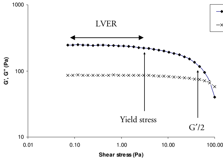
Figure 16. Rheogram of a 1.2% potato pulp suspension.
