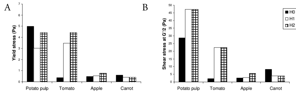
Figure 18. Yield stress (A) and shear stress at G'/2 (B) of the four fibre suspensions at an IM concentration of 1.2% following homogenisation (see Table 2 for explanations)
