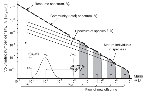
Fig. 1. Illustration of the community model: resource spectrum (with cut-off m_{cut} ) and four species size-spectra ( m_* = 2.5, 25, 250, and 2500 g) having offspring of size m_0 . Shaded regions mark the spawning stock from maturation size m_* to maximum asymptotic size M . The sum of all spectra gives the community spectrum (dashed). The spectra shown are the steady-state solutions from Andersen and Beyer (2006). Inset shows how individuals feed on smaller prey using a feeding kernel with a preferred PPMR of \beta .
