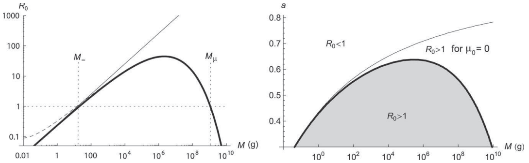
Fig. 4. (a) The reproductive success R_0 as a function of asymptotic size for a predation pressure a = 0.5 , based on the approximation (6) (thick line), based on the full solution from the appendix with background mortality \mu_0 = 0.1 \text{ year}^{-1} (dashed line) and without background mortality \mu_0 = 0 (thin line). The horizontal line is drawn at R_0 = 1 . (b) The limits to reproductive success defined by R_0 = 1 as a function of asymptotic size and predation pressure using \mu = 0.1 \text{ year}^{-1} (thick line) and \mu = 0 (thin line). The gray area shows the life histories with R_0 > 1 .
