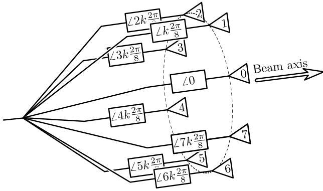
Fig. 2. Eight-element UCA with phase rotation nk2\pi/8 on element n to approximate OAM state k .
