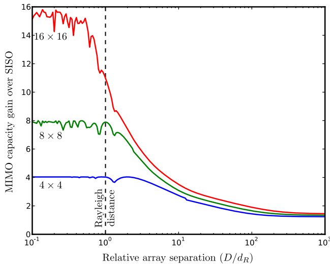
Fig. 6. Capacity gain over single antenna (SISO) system at UCA sizes 4 \times 4 , 8 \times 8 and 16 \times 16 , at an SNR of 30 dB. Curves are calculated for array radii 100\lambda and array separation distances from 10 times below to 1000 times above the Rayleigh distance ( 20.000\lambda ).
