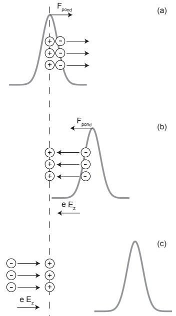
Figure 2.4. Schematic illustration of the resonance condition for plasma wave generation. Two ponderomotive “kicks” occur, one on each side of the pulse.
