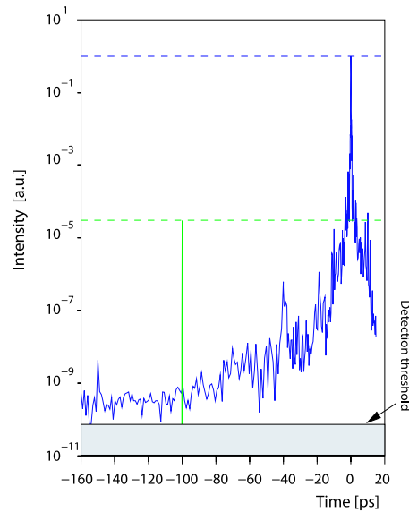
Fig. 2 Temporal intensity profile from third order autocorrelator and relative intensity level of the adjustable prepulse (illustrated for the case of 5 \times 10^{14} W/cm 2 )
