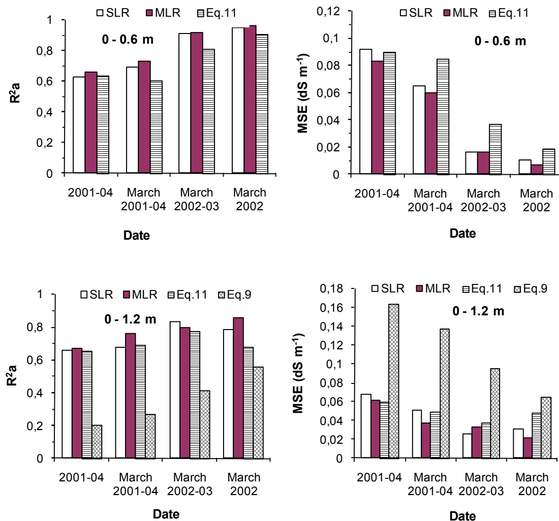
Figure 12. The R^2a and MSE of predicting LnEC_e at various soil depths (0-0.6, 0-1.2 m) and date of measurement using various models (Eqn. (9), Eqn. (11), best SLR and MLR models). For MLR, EM and plot coordinate variables were used as predictors.
