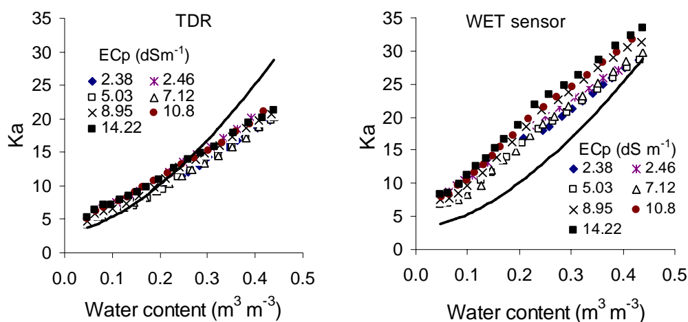
Fig. 2 The soil dielectric constant ( K_a ) measured with TDR and WET sensor vs water content ( \theta ) for each pore water electrical conductivity ( \text{EC}_p ). The solid line represents the Topp et al. (1980) equation.
