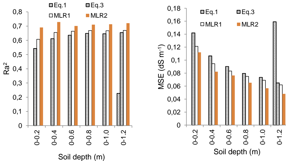
Fig. 2 Adjusted R^2 ( Ra^2 ) and mean square error (MSE) of predicting \ln ECe observed at various soil depths and seasons (12 campaigns from 2001 to 2004) with various models (equations (1) and (3), and MLR). MLR1: EM variables and plot coordinate as predictors; MLR2: same inputs than MLR1 plus groundwater properties.
