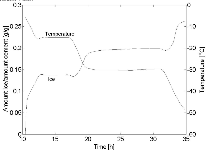
Figure 9.8.1. Amount of frozen water as function of time and temperature. Temperature held constant for 5 hours at -15^{\circ}\text{C} and 12 hours at -30^{\circ}\text{C} . Concrete with w/c-ratio 0.60 and natural air.
