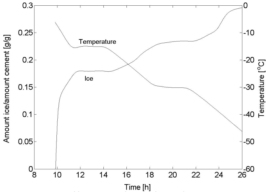
Figure 9.7.2. Amount of frozen water as function of time and temperature. Temperature held constant for 3 hours at -15^{\circ}\text{C} and -30^{\circ}\text{C} . Concrete with w/c-ratio 0.60 and 6% air.
