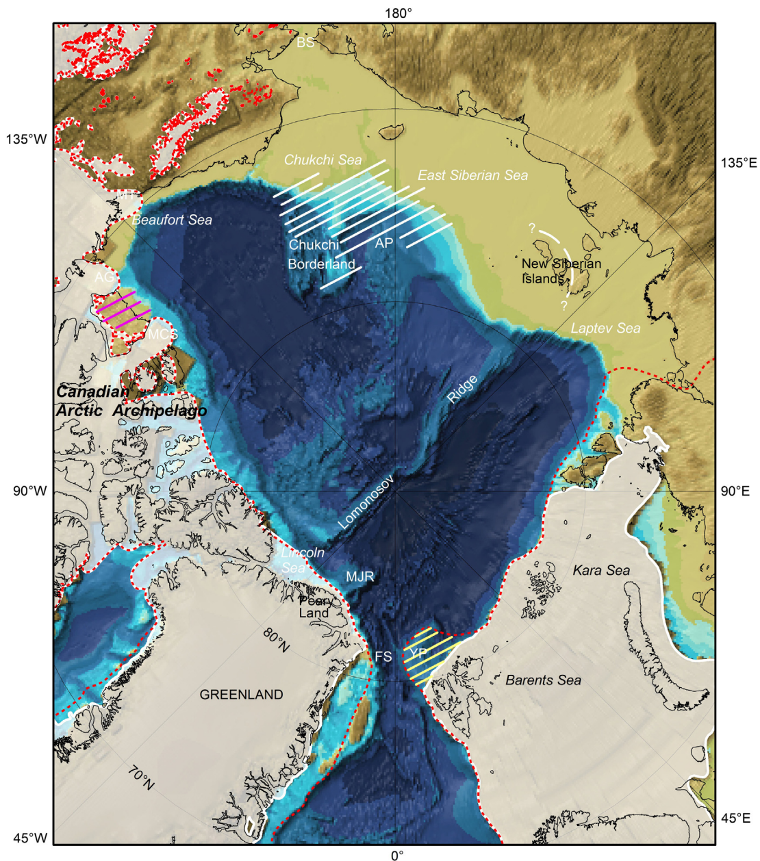
Fig. 3. Ice-sheet extension during the LGM (white semi-transparent) and Quaternary max (red dotted line). The Eurasian ice limit is from Svendsen et al. (2004a) and the Laurentide–Innuitian–Greenland is from the digital GIS files provided with the book Quaternary Glaciations – Extent and Chronology by Ehlers and Gibbard (2004). While several smaller revisions have been made to the shown ice limits, some of the more substantial revisions are indicated with cross hatching; purple (Banks Island) and yellow (Yermak Plateau). New results from the cross hatched area (white) of Chukchi Borderland – Arlis Plateau and East Siberian Sea will likely also lead to future major revisions of ice-sheet extent during the late Quaternary. The LGM topography is from ICE-5G (Peltier, 2004).
