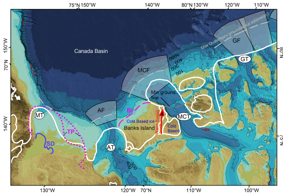
Fig. 8. Ice-sheet extension in the Beaufort Sea area during LGM inferred from Dyke (2004) (white line). The Tokerau Point Stade (TP) from Murton et al. (2010), recently suggested to represent LGM, is shown with a purple medium dashed line. The LGM ice extension on Banks Island (purple, medium dashed line), including distribution of cold respective warm based ice, is from England et al. (2009). The Sitdigi Stade (SD) is suggested to represent a re-advance during the deglaciation (see Section 3.5). Red lines indicated mapped streamlined glaciogenic bedforms as in Figs. 4 and 7. MT = Mackenzie Trough; AT/F = Amundsen Trough/Fan; MCT/F = McClure Trough/Fan; GT/F = Gustav Adolf Trough/Fan.
