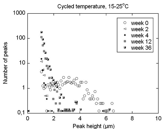
Fig. 7 Number of peaks per observation area ( 350 \times 263 \mu\text{m} ) as a function of peak height for samples stored at a cycled temperature ( 15\text{--}25^\circ\text{C} ). The number is calculated as a mean of n = 9 . The standard error of mean is \pm 1.0
