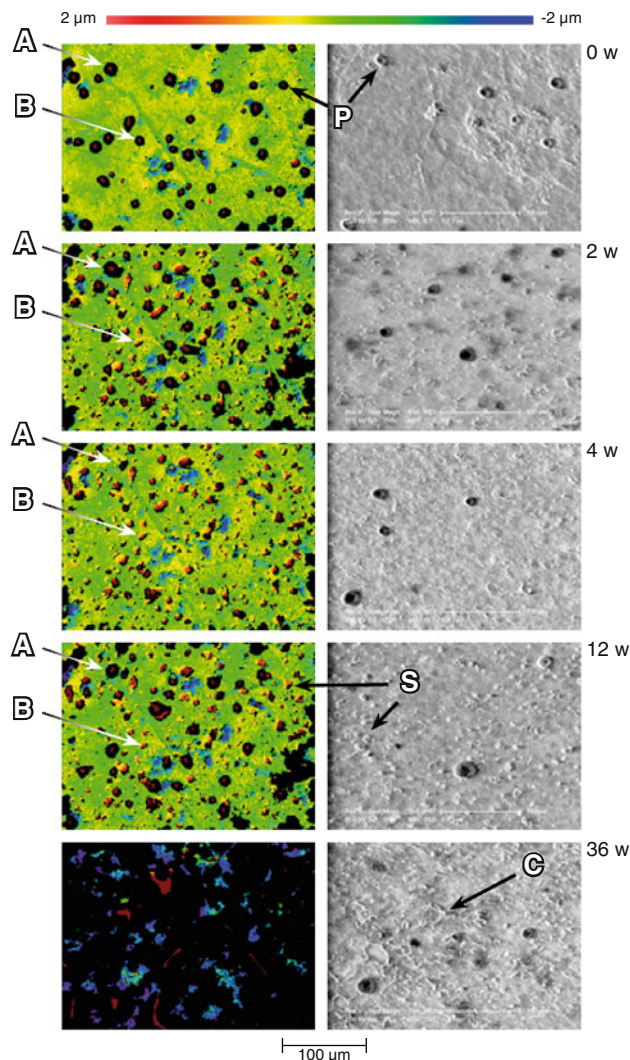
Fig. 2 Surface images of white chocolate pralines stored at a constant temperature (18 °C). Left 2D profilometry images (350 × 263 μm), produced from the same spot on the same sample, weeks 0, 2, 4, 12, 36. Some of the protrusions disappear and then re-appear (A), while some change their appearance over time (B). Right LV SEM images, from different samples, weeks 0, 2, 4, 12, 36, including protrusions (P), ridge-like topological features (S) and needle-shaped crystals (C)
