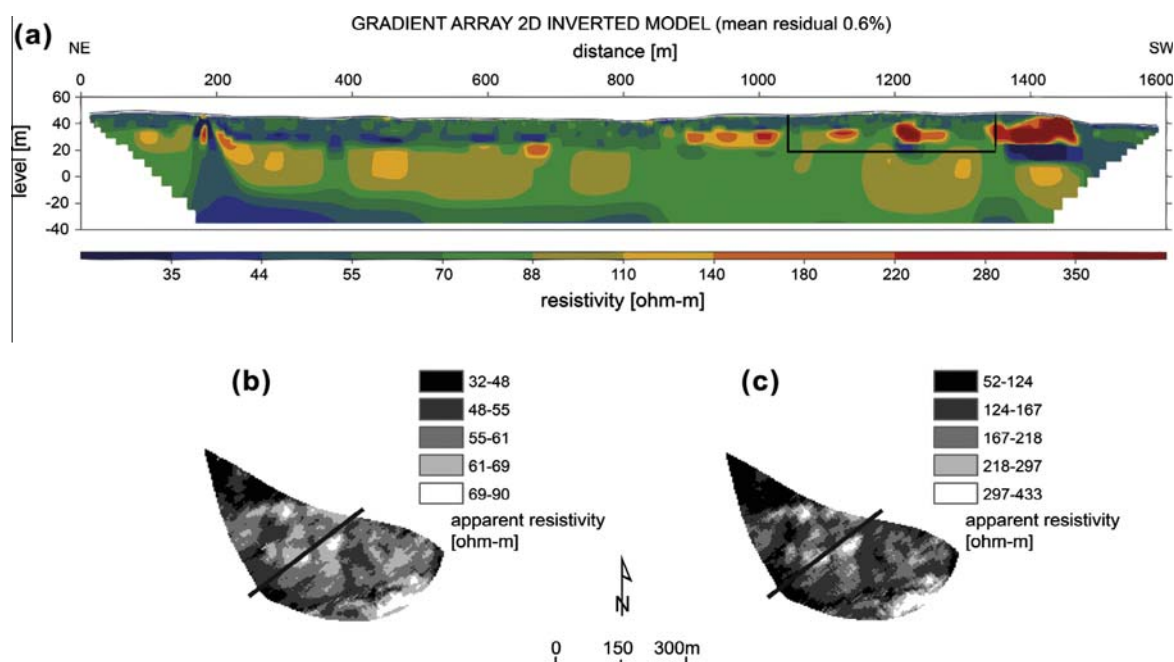
Fig. 2. (a) Inverted CVES results demonstrating electrical resistivity variability over a 1600 m long vertical 2-D transect passing through the studied catchment (boxed). (b) Results of the 27 kHz-EM-survey showing apparent resistivity variability over 0 to c. 5 m depth throughout the study area. The black line denotes the position of the CVES-transect. (c) Results of the 16 kHz-EM-survey showing apparent resistivity variability over 0 to c. 10 m depth throughout the study area. The geophysical surveys indicate the presence of a higher-resistivity formation interbedded between two lower-resistivity formations. The higher-resistivity formation is present already at 0–5 m depth as indicated by (b). The higher-resistivity formation is interpreted as a sorted, sandy deposit. The lower-resistivity formations are interpreted as clay tills.
