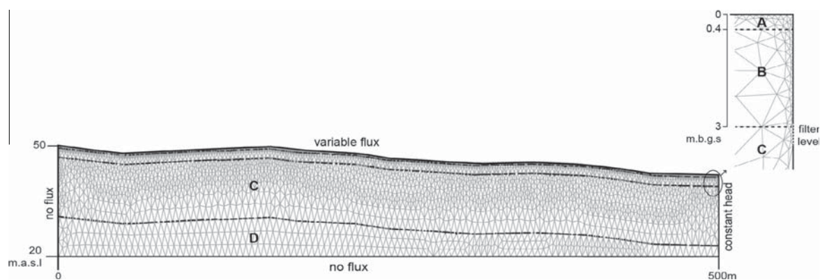
Fig. 3. Conceptual 2-D vertical model of the study area as set up in HYDRUS. The figure shows the grid mesh (grey), stratigraphic boundaries (darker), layers (letters), location and filter depth of the monitoring wells (also magnified), and boundary types (no flux/constant head/variable flux). Note that the vertical scale is exaggerated.
