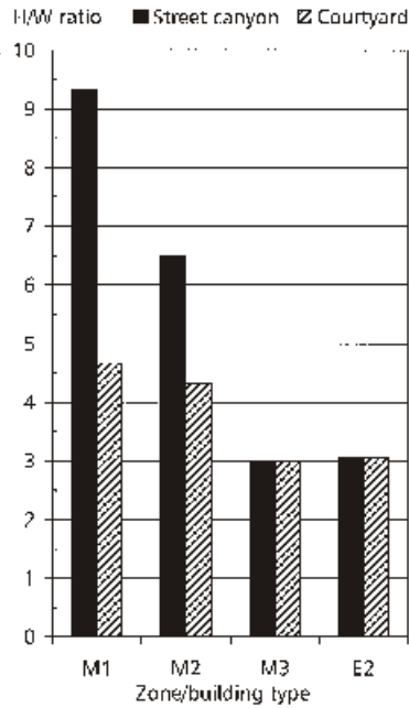
Fig. 6.23 The maximum H/W ratios of street canyons and courtyards for different housing types in the historical Medina of Fez. (Calculated from AUSF and ADER-Fez (1999), assuming street widths of 1.5, 2, 2.5 and 4 m respectively for zones M1, M2, M3 and E2).
