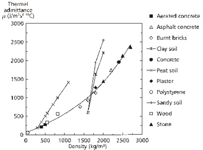
Fig. 3.2 The relation between thermal admittance \mu and density of building materials and soils. For soils, lower values are for dry soils and the higher values for saturated conditions. Sources: Evans (1980), Oke (1987) and Szokolay (2002).
