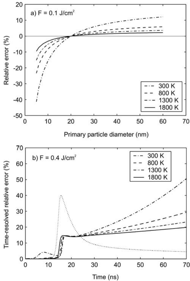
Figure 9. Influence of the gas temperature on the relative error. In a) the error for the base case is shown using gated detection (prompt 20 ns) at 0.1 J/cm 2 and in b) the time-resolved error obtained at a particle size of 30 nm with respect to a reference size at 20 nm is shown for varying gas temperature and a fluence of 0.4 J/cm 2 . Also shown is the LII signal for 30 nm particles at 1800 K. The reported laser fluence values are for the 1800 K case only. The laser fluence for the lower gas temperatures has been increased in order to attain the same maximum particle temperature for all compared gas temperatures at a given value of the primary particle diameter.
