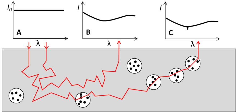
Figure 18. Schematic figure showing basic principles of gas in scattering media absorption spectroscopy (GASMAS). Light with the intensity I_0 is injected into tissue (A). If the light only encounters solid matter, there is a broad decrease in intensity (B), resulting from absorption and scattering. If the light also passes through gas-filled cavities, there is also a sharp drop in intensity in the detected light (C) in addition to the broad decrease.
