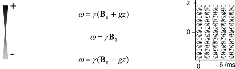
Figure 4.2 The effect of the externally applied gradient on the spin phases at different positions in the sample. The variation of the spins throughout the sample volume in z -direction can be described by a helix with pitch q^{-1} where q is defined as q \equiv \gamma g \delta / 2\pi . Figure due to Daniel Topgaard.
