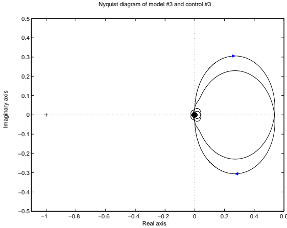
Figure 6.5 Nyquist diagram of the loop transfer-function of the combined LQR controller (with Kalman predictor) and model #3 the identified the with CVA method.
