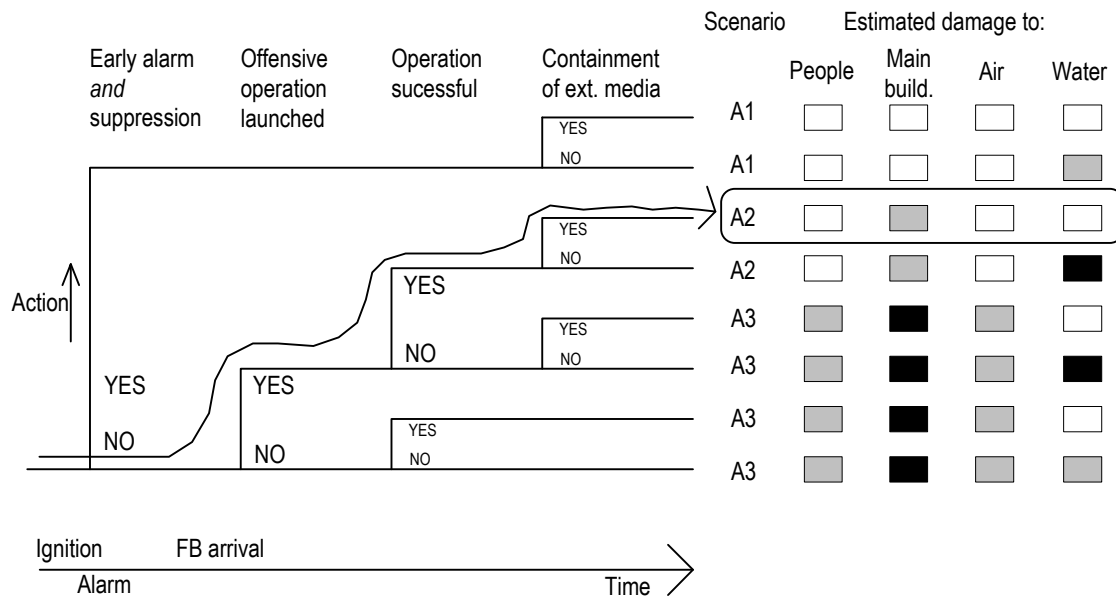
Figure 29. Each path in the event tree gives a different outcome.
