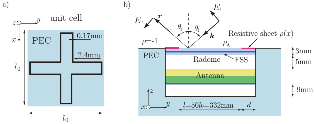
Figure 7: Geometry of the FSS bandpass radome structure. a) unit cell. b) side view with the radome and the antenna.
