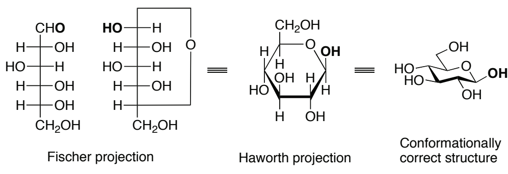
Figure 1.5 Anomeric configuration of glucose and the relationship between different projections.
