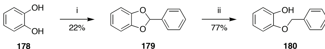
Scheme 6.17 Synthesis and opening of 179 . i) benzaldehyde dimethyl acetal, p TSA, MeCN, reflux, 18 h.; ii) BH 3 •NMe 3 , AlCl 3 , THF, reflux, 1.3 h.
