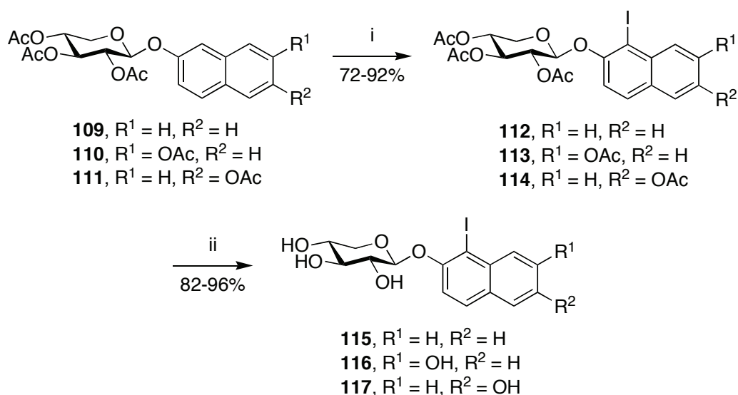
Scheme 5.5 Synthesis of iodinated naphthoxyxylosides. i) In(OTf) 3 , ICl, MS 3Å, MeCN, 1 h; ii) NaOMe MeOH, 1 h.
