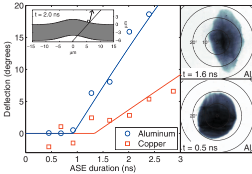
FIG. 13. (Color online) Proton beam deflection toward the laser axis as a function of ASE duration. The target is 6\ \mu\text{m} Al and Cu and the inferred ASE intensity is 2 \times 10^{11}\ \text{W}/\text{cm}^2 . As shown in the bottom right panel, the proton beam stays on the target normal axis for the shortest ASE pedestal. After shock breakout, the proton beam is steered toward the laser axis as shown in the top right panel. The inset shows the calculated shape of the foil for a 2.0 ns long ASE pedestal. The modeled emission direction (solid lines) is the calculated target normal direction at the point where the laser axis intersects the rear surface.
