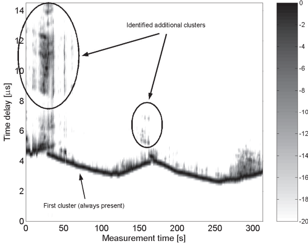
Fig. 1. An example of cluster identification for a set of consecutive power delay profile measurements performed in an urban area. Only delay bins with powers greater than -20 dB relative to that of the strongest delay bin are shown.
