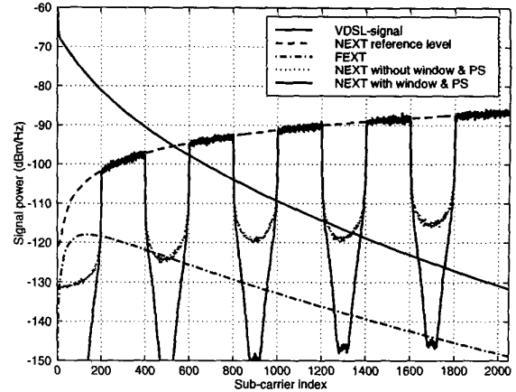
Fig. 7. Suppression of NEXT with and without pulse-shaping and windowing. Every other 200 subcarriers are used upstream.
