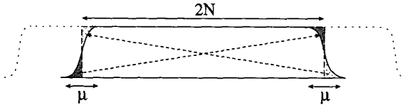
Fig. 6. Windowing the received DMT symbol.
