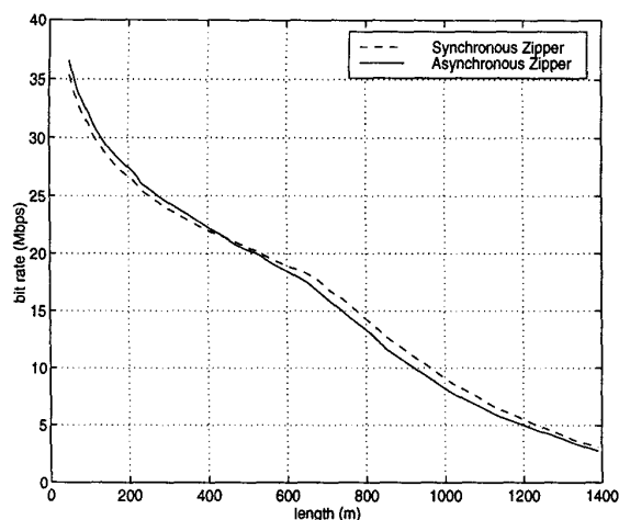
Fig. 11. Bitrate for synchronized and asynchronous Zipper, symmetrical down/up (1:1) rate.
