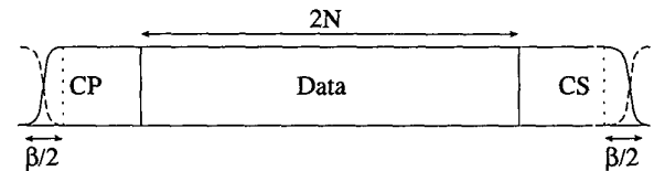
Fig. 4. Pulse-shaping the DMT-symbol in the Tx on \beta samples at each end. The CP and CS are increased in length accordingly.
