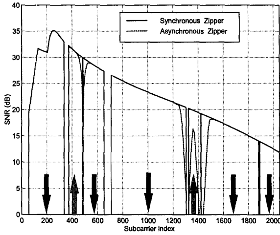
Fig. 8. SNR for asynchronous Zipper compared to synchronized Zipper for an (8:1) asymmetrical case. The arrows indicate the transmission direction.
