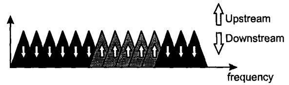
Fig. 3. Sample subcarrier assignment for asynchronous Zipper.
