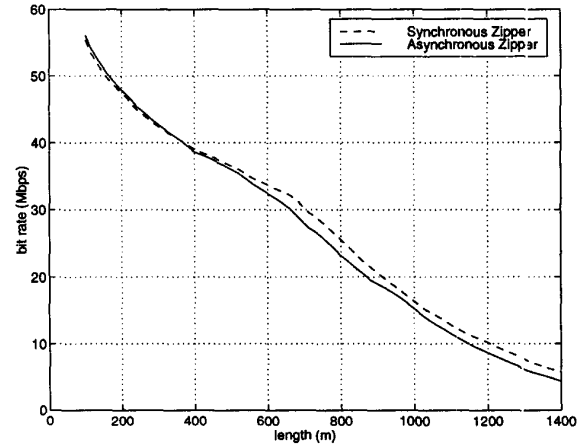
Fig. 10. Downstream bitrate for synchronized and asynchronous Zipper, asymmetrical down/up (8:1) rate.
