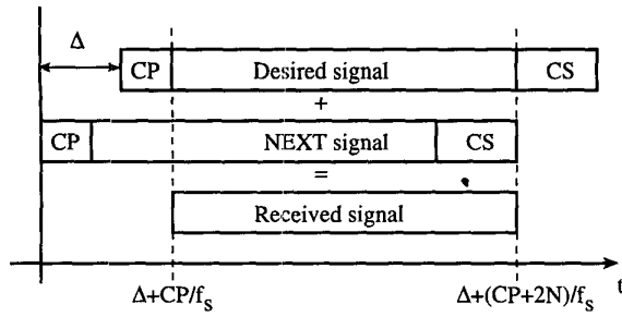
Fig. 2. Timing diagram showing the NEXT symbol frame, the desired symbol frame, and the portion of data extracted from the received frame.
