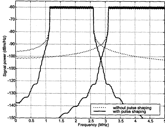
Fig. 5. Out-of-band power of two frequency bands, with and without pulse-shaping.
