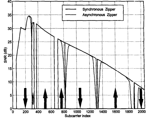
Fig. 9. SNR for asynchronous Zipper compared to synchronized Zipper for a (1:1) symmetrical case. The arrows indicate the transmission direction.
