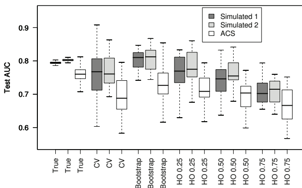
Figure III.6: Boxplots for ACS data and for Simulated data 1 and 2 using a single MLP and CV for the model selection.
