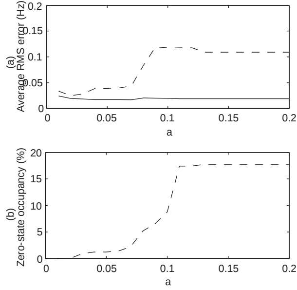
Figure 10: AF frequency tracking in QRST noise for different values of a ( \sigma^2 = 0.1 ). (a) The average RMS error at an SNR of 4 dB (solid line) and 2 dB (dashed line), and (b) the corresponding zero state occupancy.
