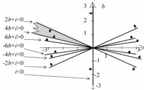
Figure 8.2 Graphical example of the Solution of the Relation System step. Here, only two free parameters, b and i , are involved. The arrows indicate in which half of the space a relation (the line) are satisfied [62].
