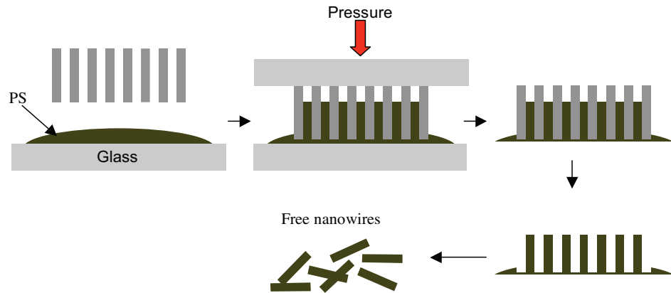
Fig. 14. The drawing shows the production of fluorescent polystyrene (PS) nanowires. An Al_2O_3 template was pressed into the DiI/PS/Xylo-solution between two glass slides. After evaporation of the Xylo, the nanowires could be scraped off from the thin plastic surface.
