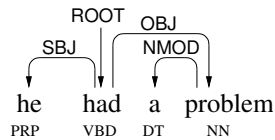
Figure 5.3: Example of features in predicate identification and sense disambiguation.
