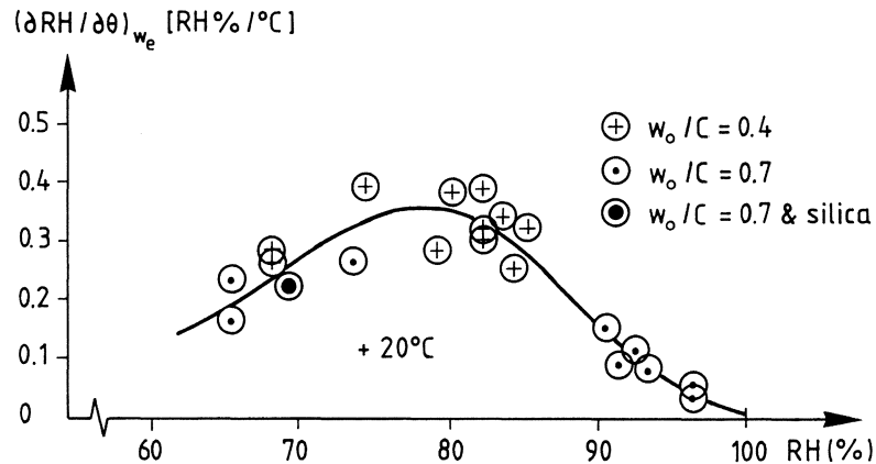
FIG 5.8 The temperature effect on the equilibrium RH in concrete. Mean temperature +20^\circ\text{C} . Nilsson (1987).
