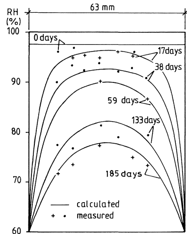
FIG 14.3 Calculated distribution of RH and measured RH during the drying of a 63 mm thick concrete specimen. w_o/C 0.6.
