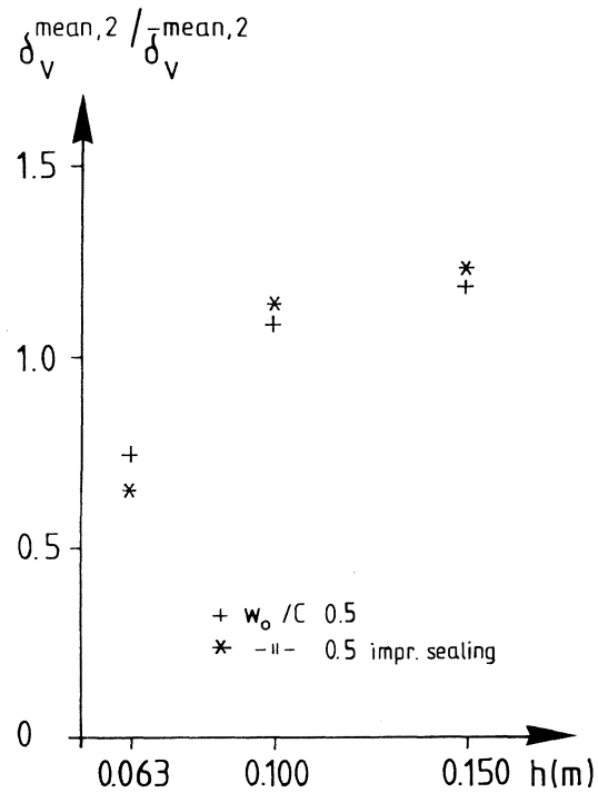
FIG 8.7 Effect of the heights of the specimens on the ratio \frac{\delta_v^{\text{mean},2}}{\delta_v^{\text{mean},2}} . The sealing between the upper box and the specimen has been improved. Cement mortar.
