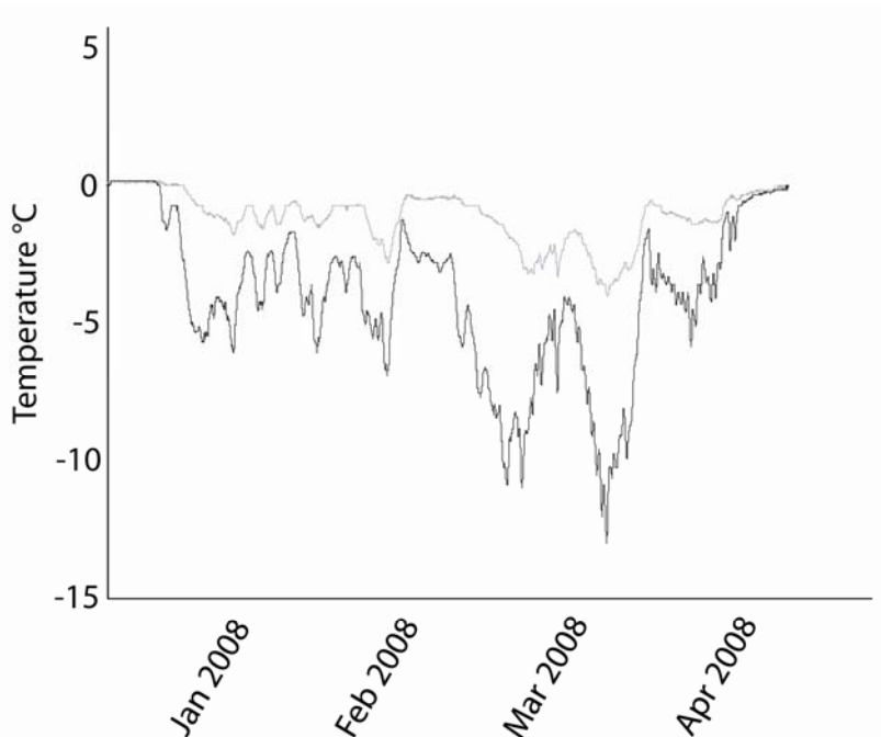
Figure 3 Ground temperatures at 15 cm depth at two individual plots, one control site (black line) and one plot with a snow fence (grey line) in spring 2008.
