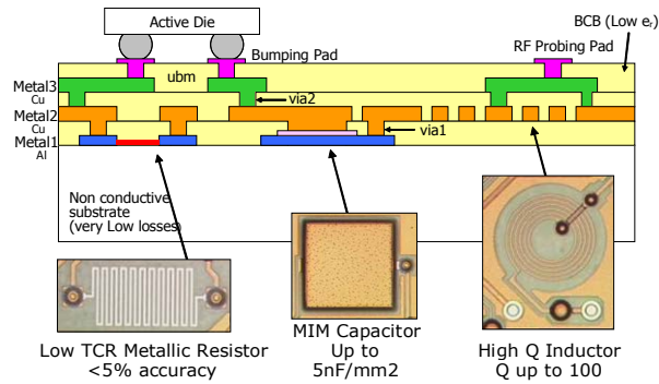
Fig. 3. Glass carrier process stack-up.
