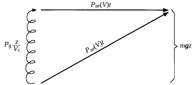
Fig. 4. A simple model for analysing the rate of climb in an initial soaring ascent that is required to yield an energetic advantage compared with a flapping-flight climb to an altitude z at some horizontal distance. During gliding flight, the bird expends a metabolic power P_g of 3BMR, where BMR is basal metabolic rate. V_c is the rate of climb when soaring, P_{ae}(V) is mechanical power during flapping flight, t is the time required to fly the horizontal distance, m is body mass and g is the acceleration due to gravity. Note that t is the same for level flight and for active climbing flight because the airspeed did not differ between these flight modes. The criterion for an initial soaring ascent to be advantageous is given in equation 3.
