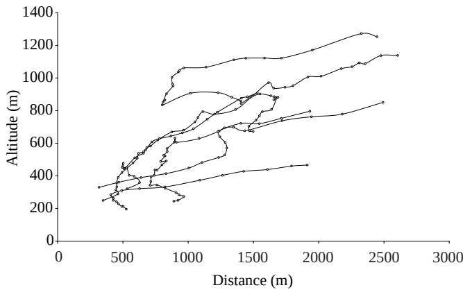
Fig. 5. A few typical tracks recorded from Eleonora's falcons with an initial soaring ascent using slope-lift close to the nesting cliffs followed by a continuing climb by active flapping flight. The distance on the abscissa is horizontal distance in the ( x, y ) plane from the bird to the observation point. The tracks illustrated had a mean climb rate of 1.49 \text{ m s}^{-1} when soaring and 1.95 \text{ m s}^{-1} when climbing using flapping flight, with an overall mean climb rate of 1.60 \text{ m s}^{-1} .
